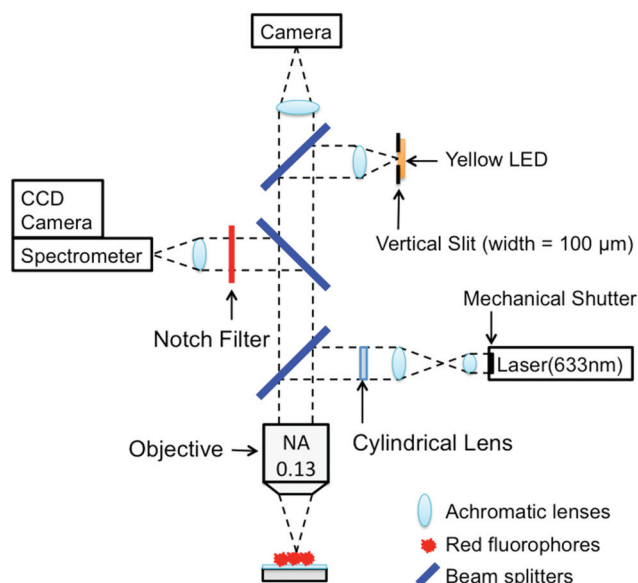
Fig. 5 Schematic illustration of the optical setup of the high-throughput imaging biosensor combining Spectral Self-interference Fluorescence Microscopy (SSFM) and White Light Reflectance Spectroscopy (WLRs). Components are not to scale.
