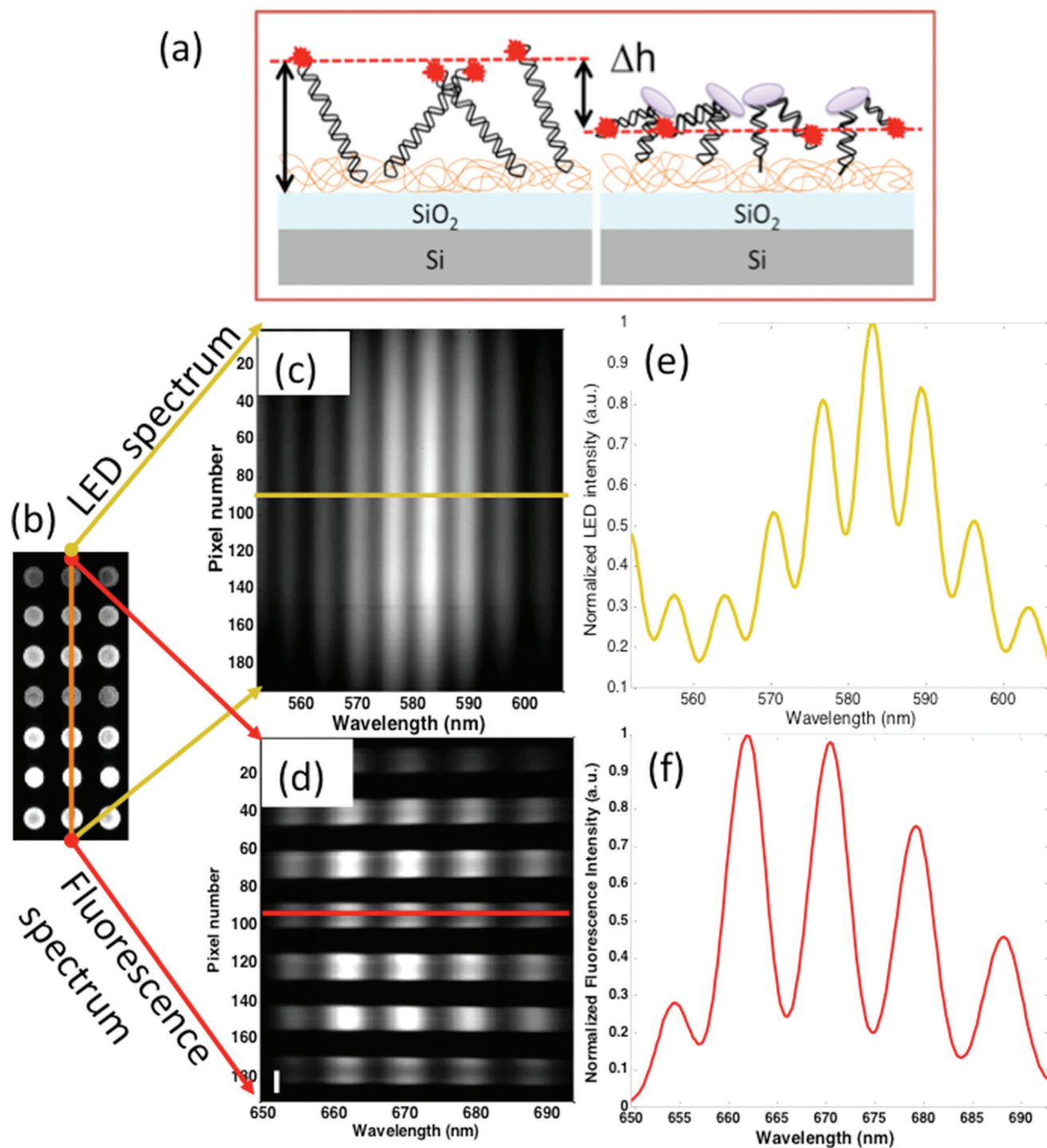
Fig. 1 High-throughput imaging biosensor combining SSFM and WLRs for simultaneous quantitation of conformational specificity and binding affinity of specific protein–DNA interactions. (a) The underlying principles of quantifying both DNA conformational change and DNA-protein binding affinity on a DNA microarray surface. The microarray substrate is functionalized with a polymeric coating (orange matrix) to form covalent bonds with DNA molecules modified with amine groups at the surface-proximal ends. The surface-distal ends of surface-immobilized DNA molecules are labeled with ATTO647N (red) fluorophores. The thickness of the DNA spot on the surface is measured by WLRs and used for obtaining the average surface density of the DNA molecules in each DNA spot. (b) A fluorescence image of a sample DNA microarray on a polymer-functionalized substrate acquired by GenePix® 4000B Microarray Scanner (Molecular Devices, LLC, Sunnyvale, CA). The orange line indicates that an image of a slit in front of an LED light source of the WLRs setup and a line of the laser of the SSFM setup overlap and are focused on a line of DNA spots at the center. (c) A one-dimensional (1-D) spectral image of an image of the LED slit focused on the microarray substrate. (d) A 1-D spectral image of the DNA spots excited by the line of laser focused on the microarray substrate. (e) A sample LED interference spectrum averaged over 10 pixels at the center of one DNA spot, indicated by the yellow horizontal line in (c). (f) A sample fluorescence interference spectrum integrated over 10 pixels at the center of one DNA spot, indicated by the red horizontal line in (d).
