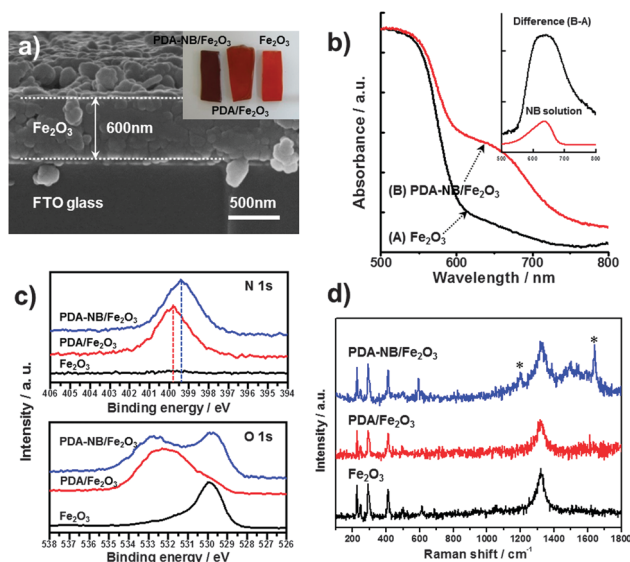
Fig. 1 Characterization of the PDA–NB coating layer on hematite. (a) SEM image of cross-section view showing the thickness of hematite film. Inset photograph shows color change of the hematite photoanode before and after coating. (b) Absorbance spectra of (A) hematite and (B) PDA–NB-coated hematite (PDA–NB/Fe 2 O 3 ), showing significant increase of absorbance in 600–700 nm, which corresponds to the absorption peak of NB solution (inset). (c) XPS spectra for N1s and O1s peaks. (d) Raman spectra of hematite, PDA-coated hematite (PDA/Fe 2 O 3 ) and PDA–NB/Fe 2 O 3 . Peaks expected from NB are indicated by asterisks.
