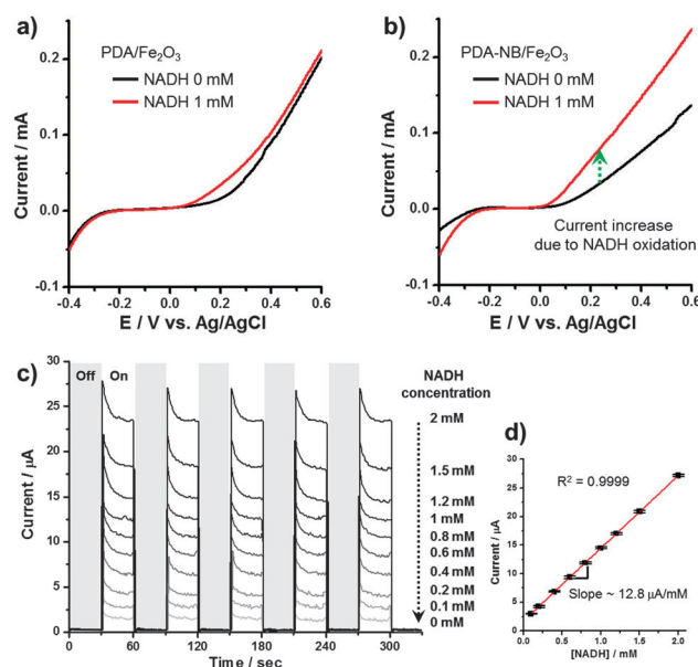
Fig. 2 Current–potential characteristics of (a) PDA/Fe 2 O 3 and (b) PDA–NB/Fe 2 O 3 with and without 1 mM NADH under visible light. (c) Photocurrent response and (d) calibration plot of PDA–NB/Fe 2 O 3 photoanode at various NADH concentrations. As the NADH concentration increases, the photocurrent increases linearly with a correlation coefficient of 0.9999.
