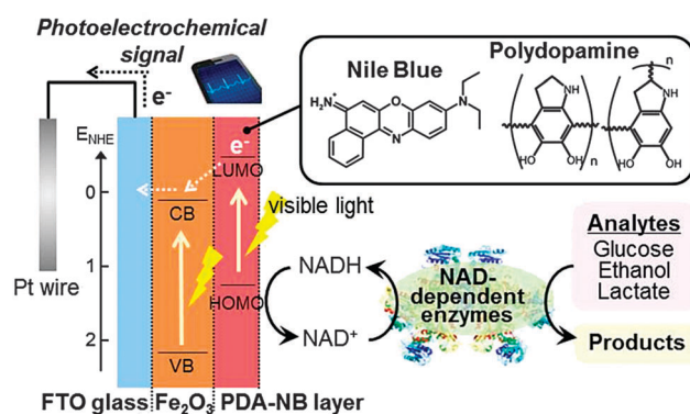
Scheme 1 Schematic illustration of the PEC biosensor platform based on the PDA-NB/Fe 2 O 3 photoanode, which is used to detect NADH and various substrates by employing NAD-dependent enzymes such as glucose dehydrogenase (GDH), alcohol dehydrogenase (ADH), and lactate dehydrogenase (LDH). A redox mediator for NADH oxidation, NB, is successfully immobilized on hematite film via PDA coating. Photocatalytic NADH oxidation by NB generates an electrical signal that is proportional to the concentration of NADH and amplified by photo-excited electrons from a hematite-based photoanode.
