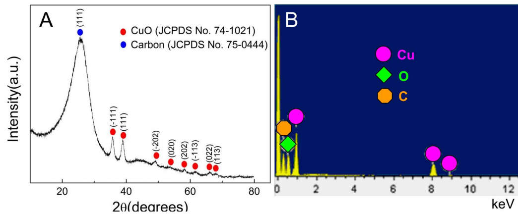
Fig. 3 XRD pattern (A) and EDS spectrum (B) of the CuO/CCF composite.
