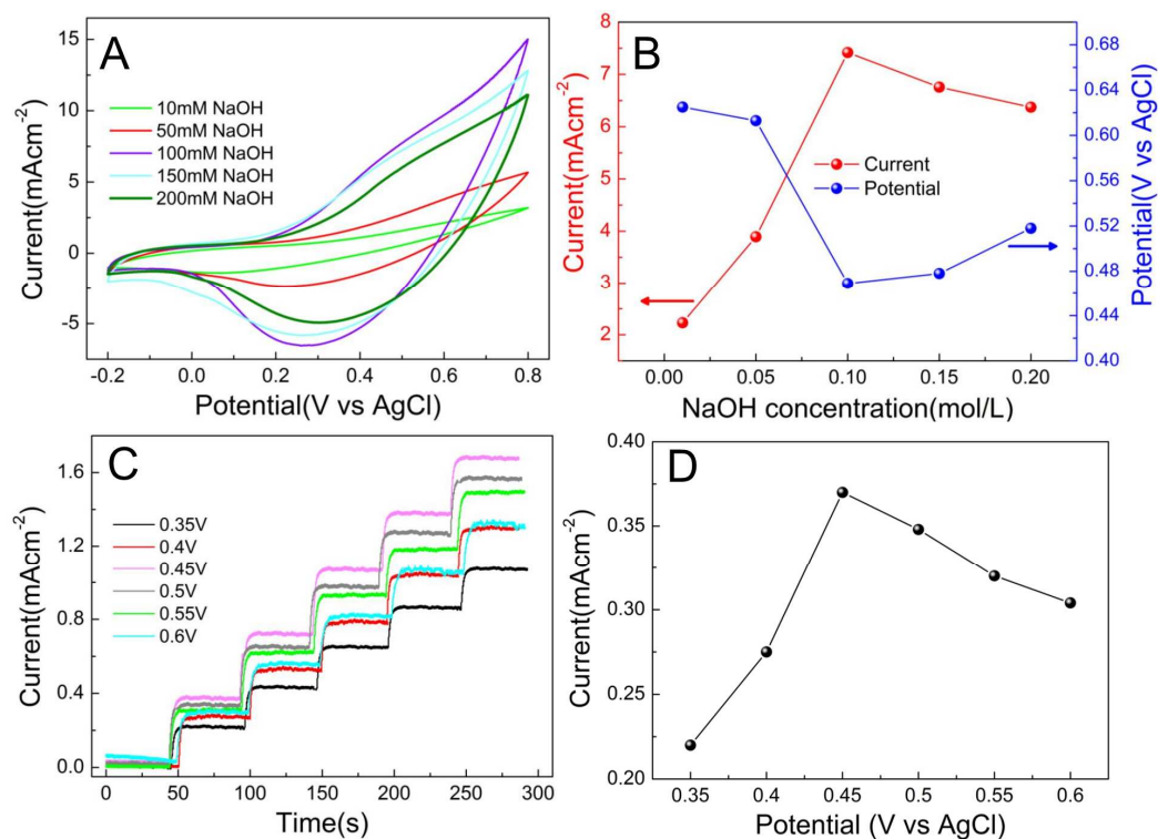
Fig. 7 (A) CVs of CuO/CFF electrode in different NaOH concentration with 1.0 mM glucose at 50 mV s -1 ; (B) effect of NaOH concentration on peak current and peak potential of CuO/CFF electrode; (C) amperometric response of CuO/CFF electrode at different potentials in 100 mM NaOH solution with a dropwise addition of 40 \mu M glucose; (D) the relationship between the current and applied potential.
