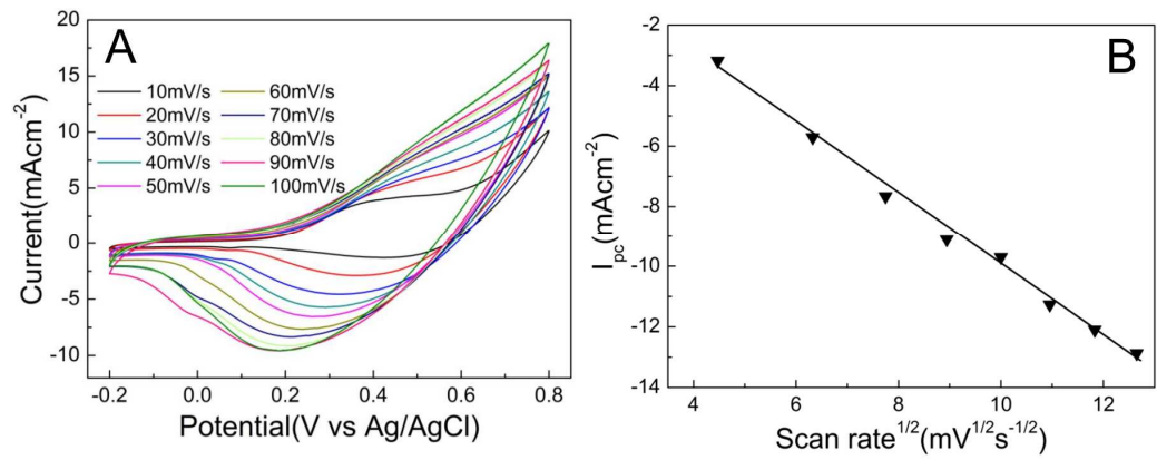
Fig. 6 CVs of CuO/CFF electrode at different scan rates from 10 to 100 mV s -1 in 100 mM NaOH solution containing 1.0 mM glucose (A); plots of cathodic peak current versus the square root of scan rate (B).
