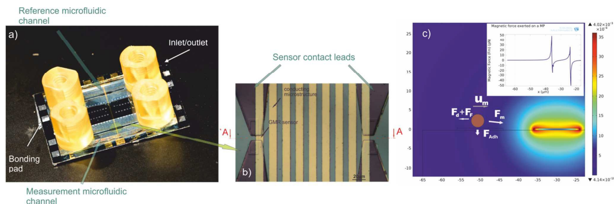
Fig. 1. a) The developed biosensor with the integrated microfluidic channels, b) microscope image upon 20x magnification; the sensor contact leads, the GMR elements and the sequential MCs are shown. c) Force analysis on a single MP, Finite element analysis of the magnetic field imposed by the current carrying MC, which attracts the MP. The view is the hypothetical cross section (A'A') of the biosensor as seen in (b). (Inset) a graph of the magnetic force exerted on the MP along the axis of motion (x). The peaks are located at the edges of the MC.
