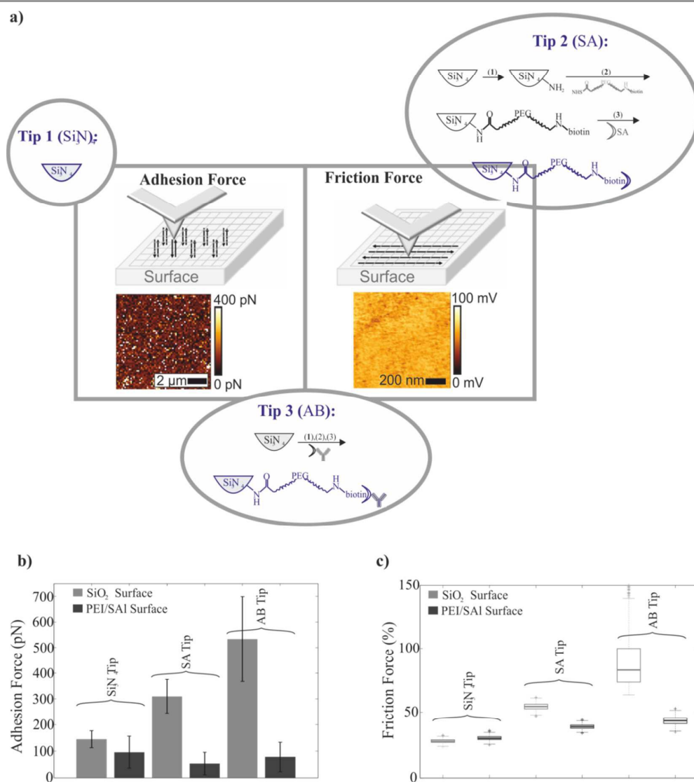
Fig. 6. (a) Chemical methods for conjugating a streptavidin (SA) monolayer and subsequently antibodies (AB) on an Atomic Force Microscope tip, in order to simulate the motion of the MPs on the modified chip's surface and measure adhesion and friction forces. The methods for acquiring the measurements for the different forces and the raw data in the form of images are displayed. (b) Adhesion force measurements with a silicon nitride tip (tip 1), a streptavidin coated tip (tip 2) and an antibody coated tip (tip 3), on a \text{SiO}_2 and a Polyethyleneimine/ Sodium Alginate modified surface. The figure clearly demonstrates the stiction of the MPs on the unmodified surface. (c) Friction force measurements using the same 3 tips and surfaces. The demonstrated difference in friction between the streptavidin coated tip and the antibodies coated one translates into velocity difference for the respective MPs during magnetophoresis.
