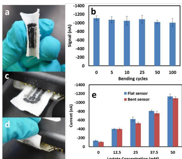
Fig. 6 (a) Mechanical bend testing of embroidered electrochemical sensors. (b) Amperometric measurements of lactate (50 mM) in PBS following up to 100 cycles of bending. Images of the sensor positioned flat (c) and bent at 90° (d) in the reader. (e) Comparative measurements of lactate using flat or bent sensors. Each bar represents the mean \pm SD of three separate measurements.
