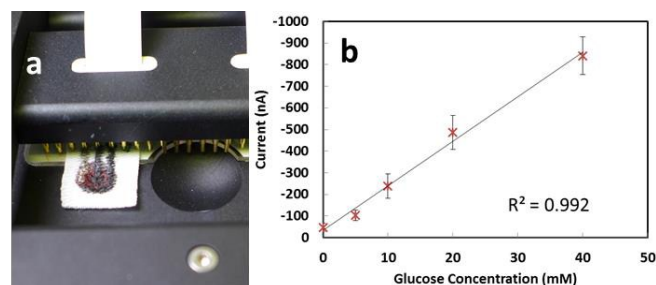
Fig. 5 (a) Embroidered sensor inside the electrochemical workstation during testing. (b) Amperometric measurements of glucose in whole blood. Values are averaged over the final 10 sec of the detection signal. Each data point represents the mean \pm SD of three separate measurements which were obtained using new sensors.
