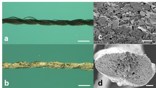
Fig. 1 Optical images of uncoated thread (a) and Ag/AgCl-coated thread (b). Scale bar, 500 µm. SEM images of Ag/AgCl-coated thread showing its surface morphology (c) and cross-section (d). Scale bar, 50 µm.
