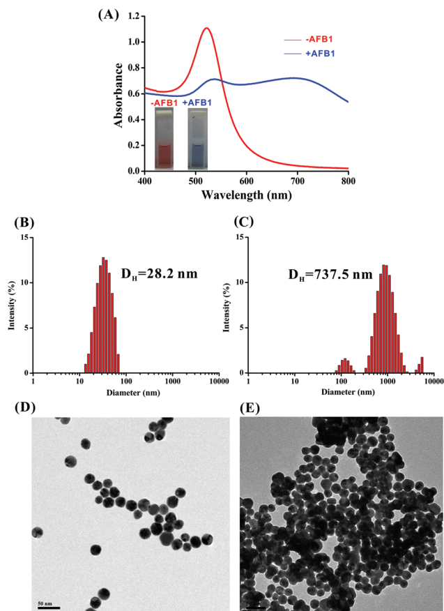
Fig. 1 (A) UV-vis absorption spectra of the colorimetric detection system in the absence and presence of AFB1 (1 \mu M). Inset: photographs of AFB1-induced color change of the Au-SA dispersion. (B) DLS measured hydrodynamic size distribution of Au-SA. (C) DLS measured hydrodynamic size distribution of the Au-SA assembly in the presence of 1 \mu M AFB1. (D) TEM image of the dispersed Au-SA. (E) TEM image of a microscopic Au-SA assembly in the presence of 1 \mu M AFB1. Scale bar: 50 nm.
