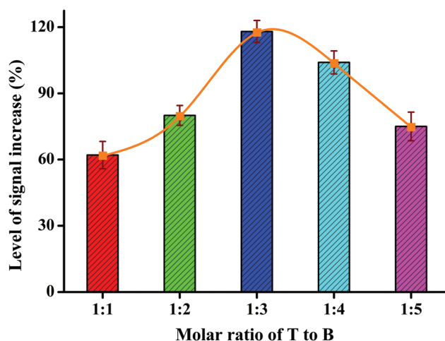
Fig. 2 Effect of the molar ratio of T to B on the response of the sensing system. The level of signal increase was plotted as a function of the molar ratio. Level of signal increase = (S - N)/N \times 100\% , where S is the signal triggered by 10 nM AFB1 and N is the signal of the corresponding negative control in the absence of AFB1. T: 100 nM, hairpin DNA: 600 nM.
