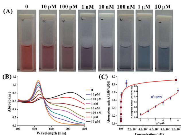
Fig. 6 (A) Photographs showing colorimetric responses of the detection system in the presence of various concentrations of AFB1. (B) Their corresponding UV-vis absorbance spectra. (C) Plots of absorption ratios ( A_{650}/A_{520} ) versus the concentration of AFB1. Inset shows the calibration curve for concentrations ranging from 10 pM to 1 \mu M. The error bars indicate the standard deviations of three replicates.
