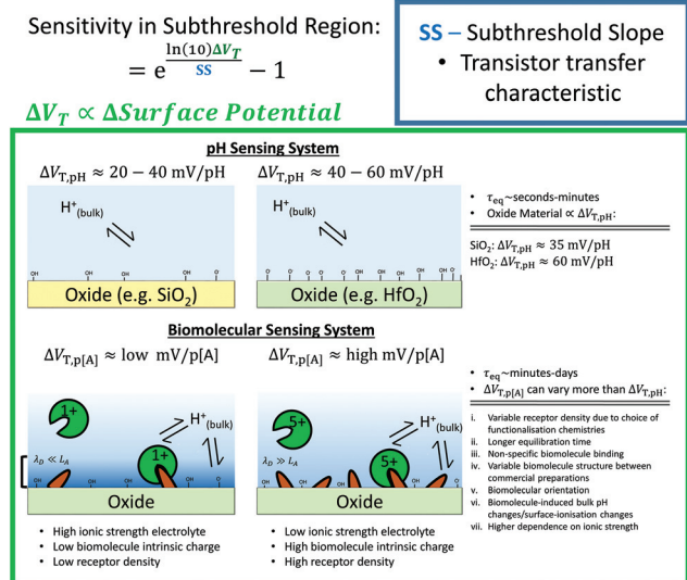
Fig. 11 Comparison of factors influencing the surface potential in a pH sensing experiment (above) with those in a biomolecular sensing experiment (below). The systems on the left and right have a low and high receptor density, respectively. Receptors for pH sensing are hydroxide groups, whereas for biomolecular detection specific receptors (shown as yellow wedges) are required. For pH sensing, the receptor density is the determining factor the change in surface potential, and therefore the shift in threshold voltage per pH ( \Delta V_{T,\text{pH}} ). In contrast, for biomolecular systems, many more factors can affect the shift in threshold voltage per 10-fold increase in concentration of analyte ( \Delta V_{T,\text{p[A]}} ). The net charge of the biomolecular system (shown as green circles) can influence response. The Debye length ( \lambda_D ) is compared to the distance of the analyte from the surface ( L_A ) on the figure, which can significantly affect BioFET signal. Here \tau_{\text{eq}} is used to refer to the typical time-scale to equilibration. The equation shown is a rearranged form of eqn (9) from the main text.
