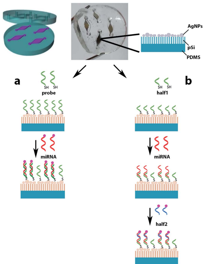
Fig. 1 Microfluidic chip integrating pSi membranes decorated with Ag NPs and the detection schemes of miRNA by (a) a one-step hybridization assay, and (b) a two-step hybridization assay.
