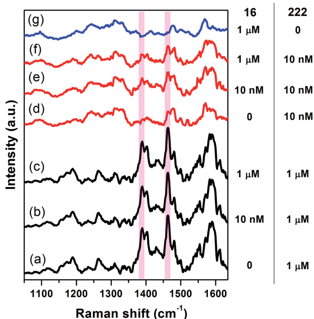
Fig. 7 SERS spectra of the PSD substrates incubated with mixtures of the target miR-222 and an interfering miR-16 at different concentrations. Curves (a), (d) and (g) represent the reference spectra of the samples incubated with 1 \mu M and 10 nM pure miR-222 alone and 1 \mu M pure miR-16, respectively. Curves (b), (c), (e) and (f) show the results of the SERS analysis of the mixtures, with the compositions being reported on the right side of the graph. The vertical bars highlight the features of half2-Cy3 at 1388 \text{cm}^{-1} and 1462 \text{cm}^{-1} .
