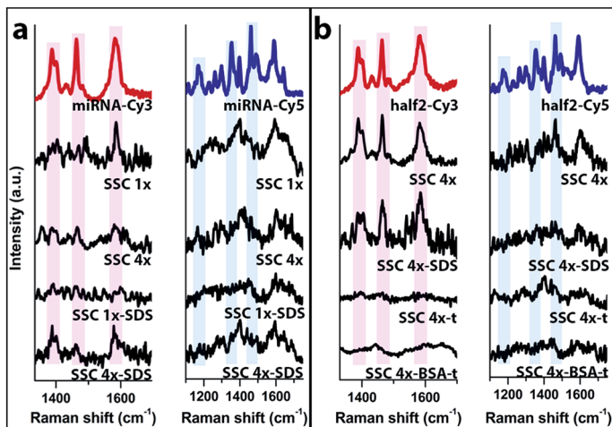
Fig. 2 (a) Evaluation of the non-specific SERS signal given by the labelled miRNA (Cy3 on the left, Cy5 on the right) incubated in the buffers used for the one-step hybridization assay (SSC 1 \times , SSC 4 \times , SSC 1 \times 0.01% SDS, SSC 4 \times 0.01% SDS) followed by washing in the same buffers; (b) evaluation of the non-specific signal given by the labelled half2 (Cy3 on the left, Cy5 on the right) incubated in the buffers used for the two-step hybridization assay (SSC 4 \times , SSC 4 \times 0.01% SDS, SSC 4 \times 0.05% Tween, SSC 4 \times 0.05% Tween 1% BSA) followed by washing in the same buffers. At the top of each series, the reference spectra of the spotted labelled target are reported. The main vibrational bands of the labels are highlighted.
