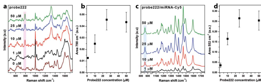
Fig. 3 Evaluation of the optimal concentration of probe222: (a) SERS spectra of the substrates incubated with different concentrations of probe222; the spectrum of a substrate pretreated with BSA is shown as a reference (brown curve); (b) integrated areas of the 790\text{ cm}^{-1} Raman peak of the probe vs. its immobilization concentration; (c) SERS spectra of the same samples after incubation with 1\text{ }\mu\text{M} miR-222-Cy5; (d) integrated area of the miRNA-Cy5 Raman peak at 552\text{ cm}^{-1} vs. the probe222 immobilization concentration. The error bars correspond to the SD.
