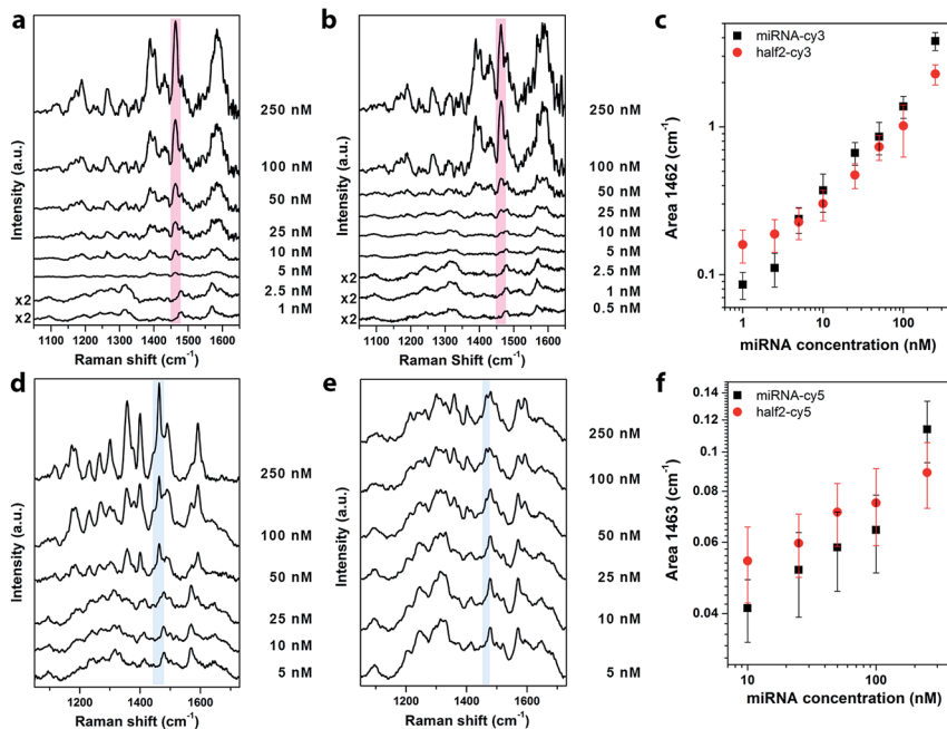
Fig. 6 (a) SERS spectra of the functionalized samples incubated with different concentrations of miR-222-Cy3; (b) SERS spectra of the functionalized samples incubated with different concentrations of miR-222 and subsequently with 1 \mu M half2-Cy3; (c) integrated area of the Cy3 peak at 1462 \text{cm}^{-1} vs. miR-222 concentration, calculated for miR-222-Cy3 (black squares) and half2-Cy3 (red dots); (d) SERS spectra of the functionalized samples incubated with different concentrations of miR-222-Cy5; (e) SERS spectra of the functionalized samples incubated with different concentrations of miR-222 and subsequently with 1 \mu M half2-Cy3; (f) integrated area of the Cy5 peak at 1463 \text{cm}^{-1} vs. miR-222 concentration, calculated for miR-222-Cy5 (black squares) and half2-Cy5 (red dots). The error bars correspond to the SD. The features of Cy3 at 1462 \text{cm}^{-1} and Cy5 at 1463 \text{cm}^{-1} are highlighted.
