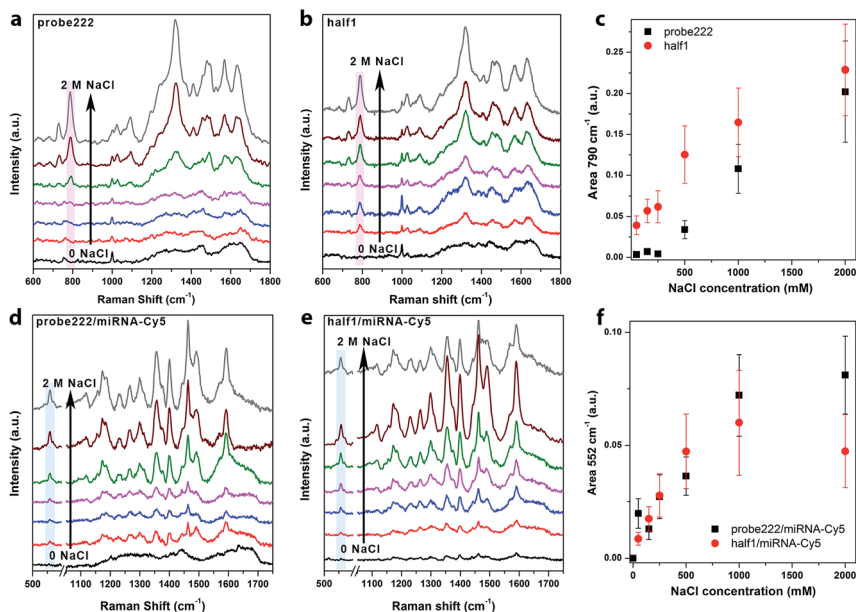
Fig. 5 Evaluation of the optimal ionic strength in the immobilization buffer: (a) SERS spectra of probe 222 (25 \mu M) incubated at different NaCl concentrations; (b) SERS spectra of half1 (10 \mu M) incubated with different NaCl concentrations; (c) integrated areas of the 790 \text{cm}^{-1} Raman peak of probe222 (black squares) and half1 (red dots) vs. the NaCl concentration; (d) SERS spectra of the samples in (a) after incubation with 1 \mu M miR-222-Cy5; (e) SERS spectra of the samples in (b) after incubation with 1 \mu M miR-222-Cy5; (f) integrated area of the miRNA-Cy5 Raman peak at 552 \text{cm}^{-1} vs. the NaCl concentration for the samples functionalized with probe222 (black squares) and half1 (red dots). The error bars correspond to the SD.
