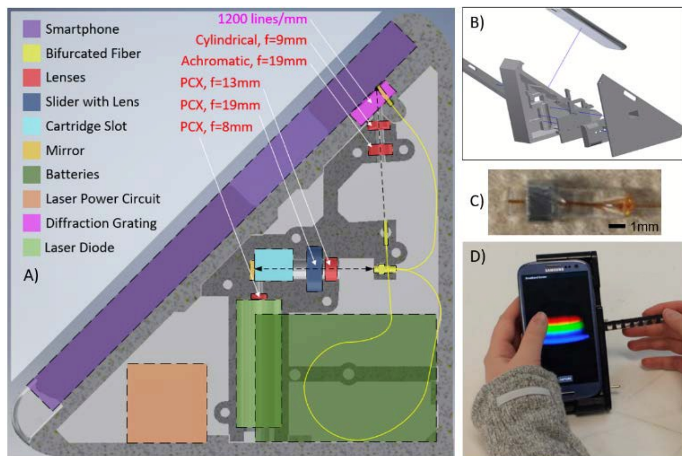
Figure 1. Design of Spectral TRI-Analyzer. A) Schematic of internal layout for optical and electrical components. A custom bifurcated fiber (100 \mu\text{m} core with d=1.8 mm glass capillary tube (proximal) and 2 \times d=1.25 mm ceramic ferrules, Coastal Connections) was used to compact the light path into a handheld device. Fiber is arranged to maximize bend radius, increasing long-term stability. B) 3D CAD model was created, comprised of 5 plastic parts printed via stereolithography. Two halves of optical housing maintain lens alignment and optical chamber isolation. All portions of cradle were designed to slide together and attach with M3x0.5 machine screws. C) Glass capillary tube with bifurcated fibers and metal nut used to align the fiber in the cradle. D) Image of final device in use with absorption cartridge.
