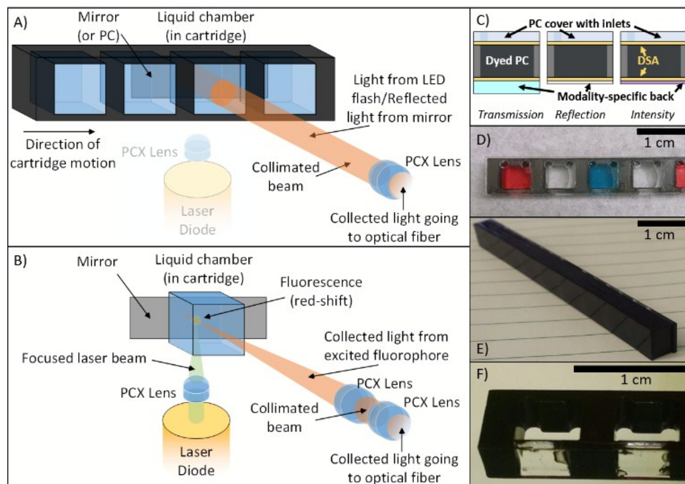
Figure 2. Two principal light paths and cartridges for each of the three modalities. A) Reflection (PC-only) and Transmission (absorption or PC) optical pathway. Collimated light from the on-board smartphone flash is directed through the sample chamber. For reflection-based PC measurements, a back-coated cartridge prevents transmitted light from being collected. For transmission measurements, light is reflected by cradle mirror directed toward the collection fiber. B) Fluorescence/Luminescence Intensity optical pathway. A laser pointer diode is co-focused to a point near the back-side of the cartridge where the collection fiber is similarly focused via addition of a single plano-convex lens into the optical path via a SLA-printed slider actuated from outside the cradle. Additional cartridge wells/housing was removed for clarity in B). C) "Sandwich" style cartridge fabrication alternating plastic or glass substrates with double-sided-adhesive (DSA) showing how different backings facilitate different modalities. D) Transmission cartridge showing inlet/outlets and optically-isolated chambers. E) Dyed PC for label-free Reflection measurements. F) Close-up of Intensity cartridge demonstrating selectively-dyed cartridge body allowing for bottom-illumination with 532 nm laser diode.
