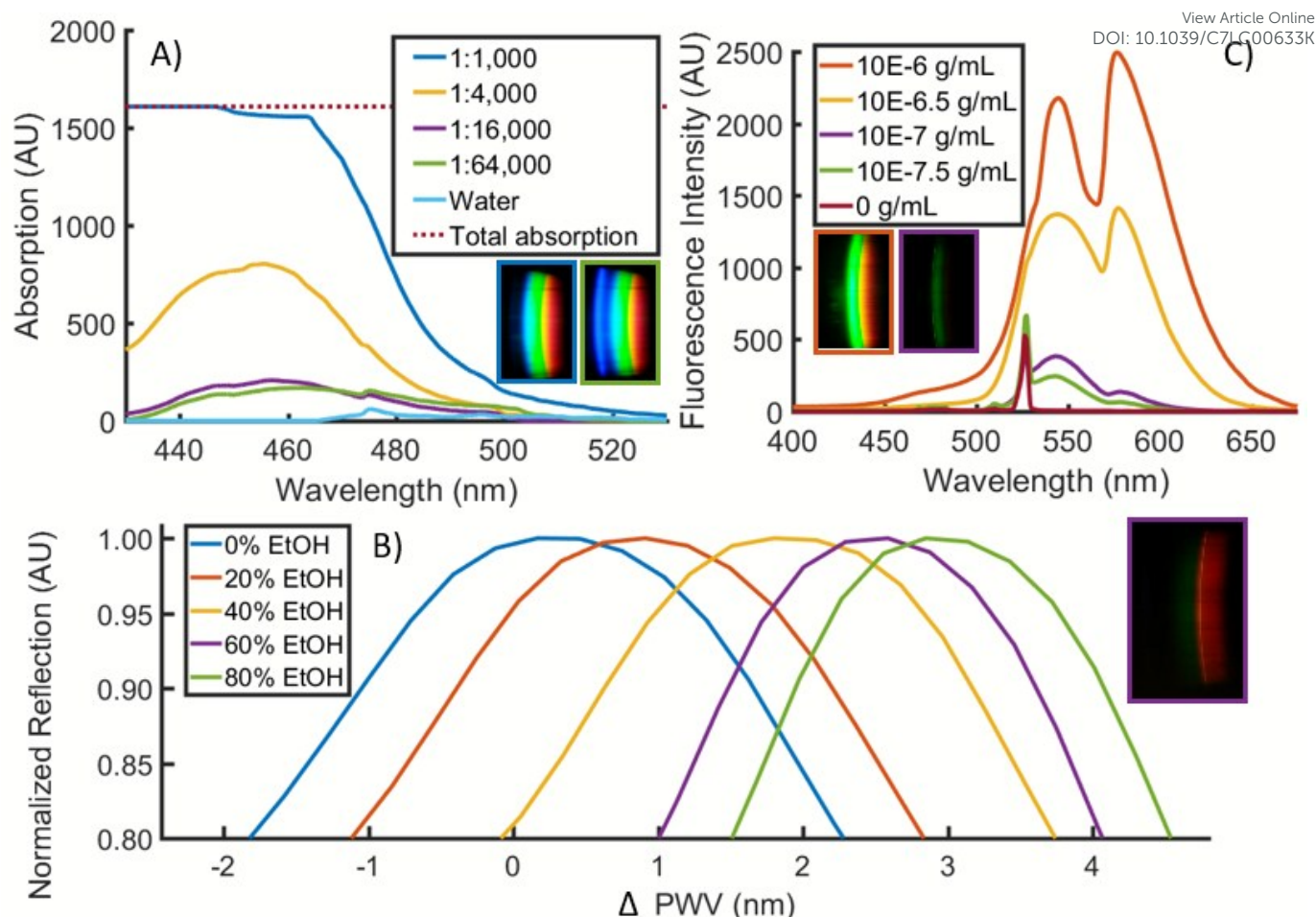
Figure 3. Qualitative proof-of-concept of 3 principal modalities. A) Transmission. Yellow food dye was diluted in water at concentrations ranging from 1:1,000 to 1:64,000, a 64x concentration range. Absorption was measured by subtracting sample transmission from that of water. Observable absorption occurred in the blue region (400–500 nm) of the spectrum. Inset raw images correspond to concentration of yellow dye of their outline. B) Reflection. 0–80% mixtures of ethanol in water were prepared and introduced into a PC-based cartridge, producing narrowband reflection in the 580 nm range. Measurements of each cartridge chamber filled with water were subtracted from measurements of those chambers filled with ethanol solutions to produce \Delta PWV shifts. Inset raw image corresponds to concentration of ethanol of its outline. A central line of pixels was used to produce spectra shown. C) Intensity. R6G dye was diluted in water and excited with the on-board laser diode. Inset raw images correspond to concentration of R6G of their outline.
