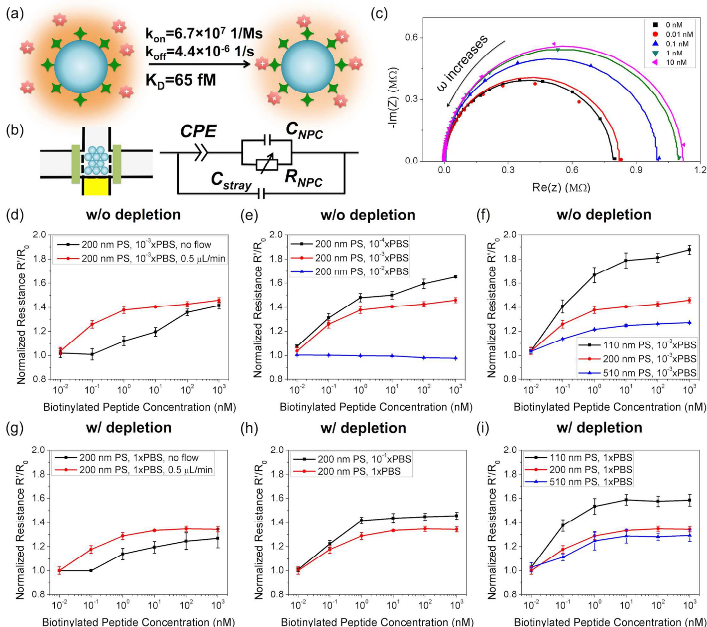
Figure 4. Detection of a biotinylated positively charged peptide (GRGGRG). (a) Schematics of the biotinylated peptide detection. (b) Equivalent electrical circuit diagram of the device. (c) Complex impedance plot of the chip at different concentrations of peptide ( 10^{-3} \times \text{PBS} , without depletion). (d-f) Detection of the peptide in low ionic strength buffers without depletion. (g-i) Detection of the peptide in high ionic strength buffers with depletion. Samples were injected at a flow rate of 0.5 \mu\text{L/min} for 15 min, unless otherwise specified.
