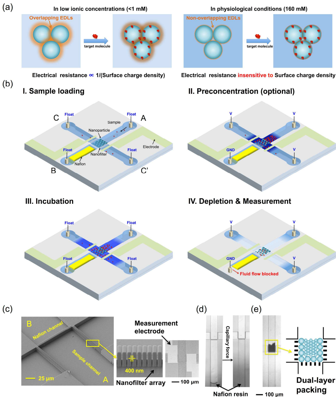
Figure 1. Principle and design of the nanofluidic biosensing platform. (a) Electrostatic effect-based nanofluidic biosensing does not work in normal physiological conditions due to the suppression of the Debye length at high ionic concentrations. (b) Principle of ion concentration polarization coupled nanofluidic crystal for biosensing. (c) SEM image of the central sensing region on the silicon substrate, a magnified view of the nanofilter array, and bright-field microscope photo of the chip after anodic bonding, which shows the micropatterned Ag/AgCl electrode pair on the glass
