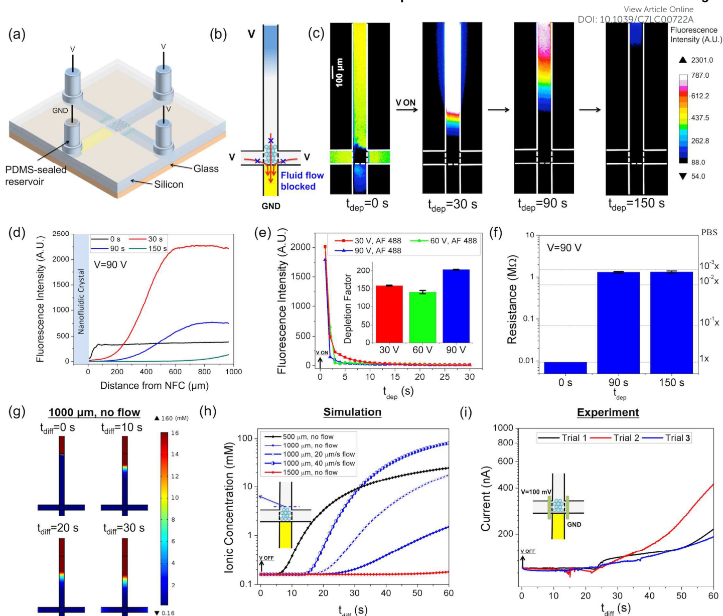
Figure 2. Characterization of the ion depletion effect. (a) Configuration of the device. (b) The electroosmotic flow was mechanically blocked, forcing the ion depletion zone to continuously grow. (c) Fluorescence images of the ion depletion process using 50 \mu\text{M} Alexa Fluor 488 in 1 \times PBS. (d) Fluorescence profile along the channel at different times shown in (c). (e) Fluorescence intensity and depletion factor in the vicinity of the NFC over time. 400 \mu\text{M} Alexa Fluor 488 in 1 \times PBS was used for the measurement. (f) Electrical resistance of a 510 nm NFC after different time lengths of depletion at 90 V. (g) COMSOL simulation of the back diffusion process of ions over time, when the depletion zone is 1000 \mu\text{m} long. (h) Simulated concentration in the vicinity of the central zone during the back diffusion of ions, at different initial depletion lengths and flow rates. The fluid flow is mainly caused by the uneven fluid levels in different reservoirs. (i) Electrical current through a 200 nm NFC during the back diffusion of ions. 100 mV was applied between the micropatterned Ag/AgCl electrode pair.
