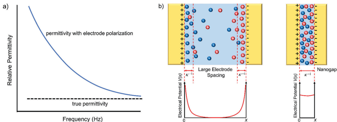
Fig. 1 (a) Effect of electrode polarization on measurements of the electrical relative permittivity and (b) overlapping electrical double layers leads to a constant electrical potential across a nanogap device, eliminating electrode polarization effects.
