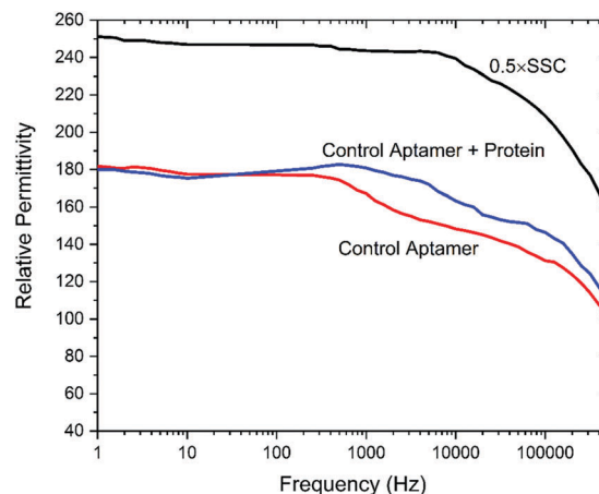
Fig. 7 Relative permittivity vs. log (frequency) for a bare nanogap device in the presence of a 0.5 \times \text{SSC} buffer (black curve), after surface functionalization with a control (non-binding) single strand DNA aptamer (red curve), and after exposure to human \alpha -thrombin protein (concentration 1 \mu\text{M} in 0.5 \times \text{SSC} buffer solution). In this case, the immobilized control oligomer is incapable of forming the active G-quadruplex structure with the protein so hybridization should not occur.
