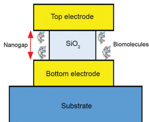
Fig. 2 Schematic of the biosensor device structure consisting of top and bottom gold electrodes separated by an etched SiO 2 support layer. Binding of biomolecules to the aptamer functionalized electrodes modifies the impedance between the top and bottom electrodes.
