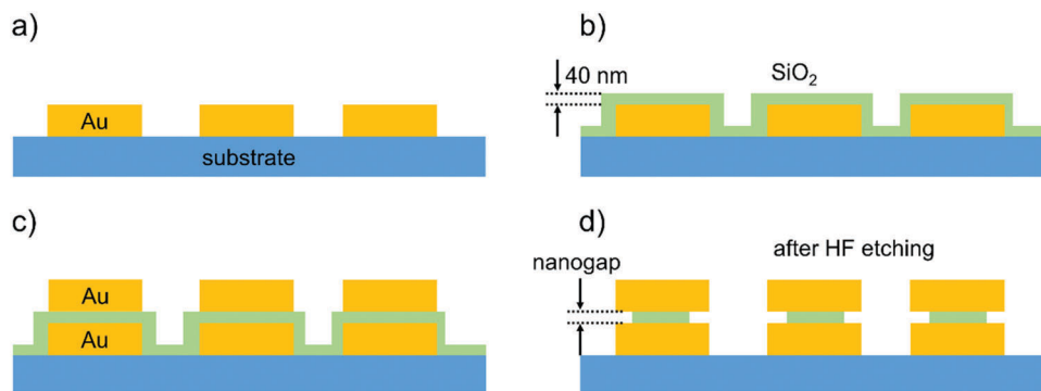
Fig. 3 Fabrication steps used to construct the biosensor. (a) Deposition of the bottom electrode using standard photolithography with a metallization and lift-off process, (b) deposition of a 40 nm thick \text{SiO}_2 layer by RF magnetron sputtering, (c) deposition of the top electrode using photolithography, and (d) HF etching of the \text{SiO}_2 layer to form the nanogap space between the two electrodes.
