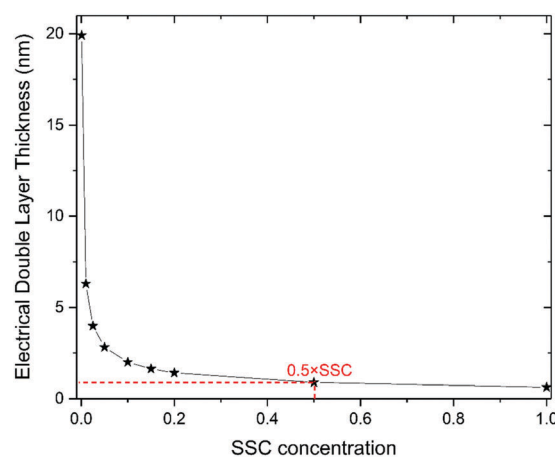
Fig. 8 Electrical double layer thickness vs. concentration of the SSC buffer determined from numerical calculations based on the Extended Debye Hückel model and Davies equation.
