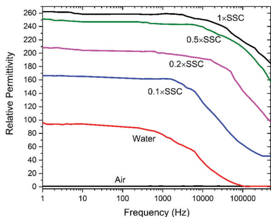
Fig. 5 Relative permittivity as a function of log (frequency) for various concentrations of SSC buffer solution ranging from 0.1 \times \text{SSC} (blue), 0.2 \times \text{SSC} (magenta), 0.5 \times \text{SSC} (green) and 1 \times \text{SSC} (black). Also shown are curves for de-ionized water (red) and air (black).
