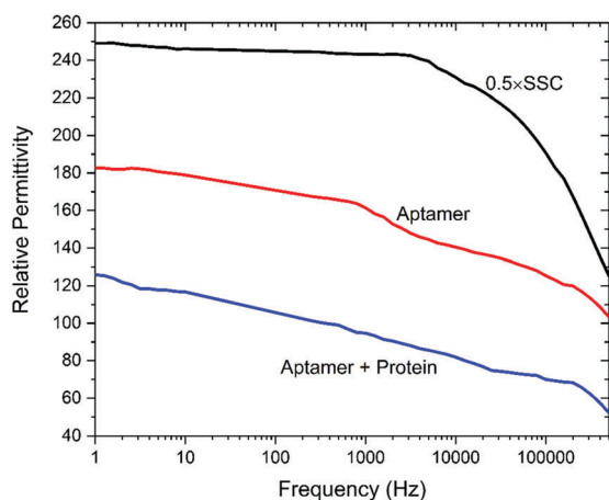
Fig. 6 Relative permittivity vs. log (frequency) for a bare nanogap device in the presence of a 0.5 \times \text{SSC} buffer (black curve), after surface functionalization with the single strand DNA aptamer (red curve), measured again in 0.5 \times \text{SSC} buffer, and after binding with human \alpha -thrombin protein (concentration 1 \mu\text{M} in 0.5 \times \text{SSC} buffer solution).
