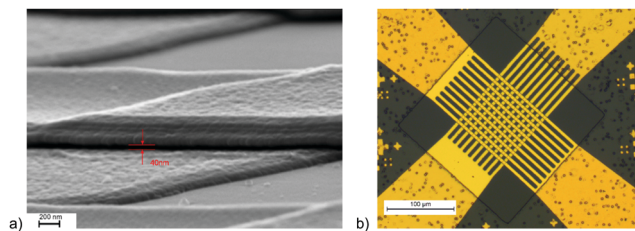
Fig. 4 (a) SEM image of the etched region of the nanogap biosensor confirming a 40 nm etched gap separates the top and bottom electrodes. (b) Optical image of the final nanogap sensor consisting of 10 by 10 overlapping crossbar electrodes to form 100 active capacitors in parallel. The outer region of the device (dotted) is a protective resist so that only the active sensing region comes into contact with the solution.
