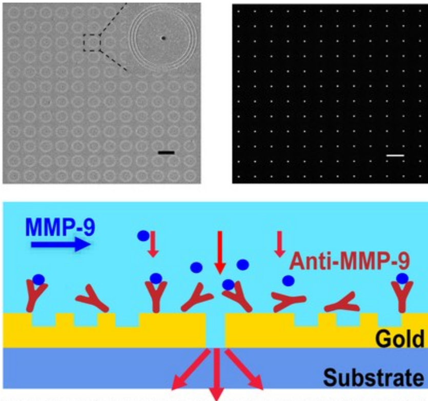
Nanoplasmonic interferometric imagers successfully detect MMP-9 in supernatant, demonstrating the potential for multiplexed sensing for cell function analysis.
