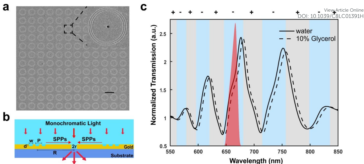
Figure 1 The principle of operation of a single circular plasmonic interferometer. (a) A SEM image of the 12×12 interferometer array. Scale bar= 12.5 μm. Inset is a magnified SEM image of a single interferometer showing the ring-hole structure. (b) Side view of the nanoplasmonic device and propagation of two interfering components. (c) Transmission interference spectra under white light illumination when the surface is exposed to water (black line) and 10% water-glycerol (black dashed line) mixture. The grey/blue shaded areas denote the range of wavelength within which the intensity change is positive(+) or negative(-) with exposure to 10% glycerol compared to water. The red shaded-area denotes the spectral line shape of a red LED used as the illumination source.
