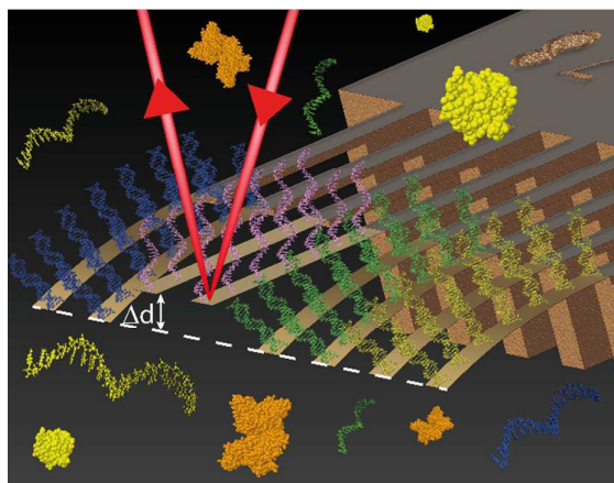
Fig. 1. Illustration of target binding on the cantilever array surface. Perspective is from inside the fluidic chamber. The laser from the optical beam read out detection method is shown reflecting away from a cantilevers surface, out of the chamber and towards the detector. Differential deflection ( \Delta d ) arise between the in-situ reference probes (pink) and target sensitive probes (blue, green and yellow), four times two sensors each. Targets are captured via specific nucleic acid hybridisation on the densely packed oligonucleotide receptor layer on the top side of the sensor array. Steric hindrance of the hybridised targets on the higher populated probe sensors build-up of stress and cause a downward bending. Low concentration of proteins, globulin (yellow) and albumin (orange), are also depicted to indicate measurements in serum or plasma. The dimensions of the objects shown is not drawn to scale.
