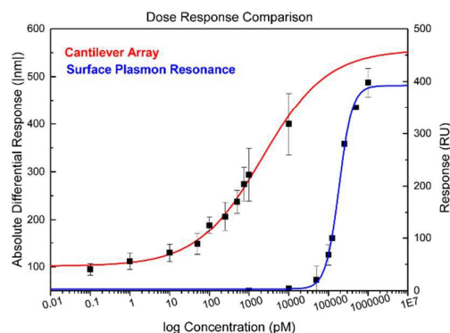
Fig. 2. Dose response comparison cantilever array versus SPR. Summarised SPR hybridisation data obtained using Biacore sensor chip functionalised with 1 \mu M thiolated probe for 1 hour. A logistic model was applied and a sigmoidal fit plotted. SPR measurements had to be conducted in pure nucleic acids spike in solutions as measurements in cell lysate were not possible due to a complete masking of the miRNA concentration signals by the lysate proteins. Error bars include chip to chip variabilities and intra chip results. Cantilever array annealing data obtained from ten miRNA target spike-in concentration experiments in Me15 cell lysate background in flow-through conditions (see methods). Error bars are calculated using the standard deviation from three measurements. As observed the dynamic range of the cantilever based technology is larger than the one from the surface plasmon technology.
