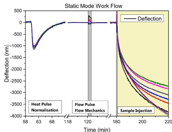
Fig 5. Automated workflow of cantilever experiments. First, a temperature pulse (+2°C) is induced at 60 minutes for 12 seconds to allow for subsequent mechanical normalisation between cantilevers in one array. The cantilevers bend depending on their individual bimetallic coating, a narrow distribution indicates mechanical conformity. Then, a flow pulse (38 µl at 150 µl/min) at 120 minutes as a control experiment reveals any flow induced motion. Laminar streaming causes the cantilevers deflection. The sensors should immediately come back to the base line after the flow pulse if the flow is not altering the mechanics of the sensor. Then 38 µl at 150 µl/min of miRNA containing samples are injected and the raw data of the sensors are recorded while the solution in the fluid chamber is again stopped (yellow background). White background indicates no flow, grey areas depict buffer flow and the yellow background illustrates sample incubation.
