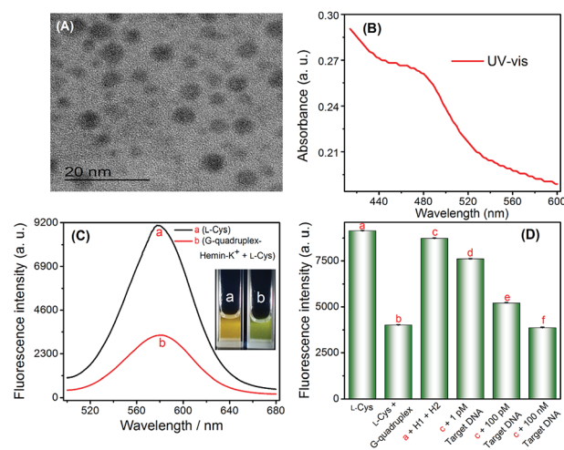
Fig. 1 (A) TEM of CdTe QDs, (B) UV-vis spectrum of CdTe QDs, (C) fluorescence spectrum under different conditions. (a) L-Cys only; (b) G-quadruplex-hemin- K^+ + L-Cys, (D) experimental feasibility verification under different conditions.
