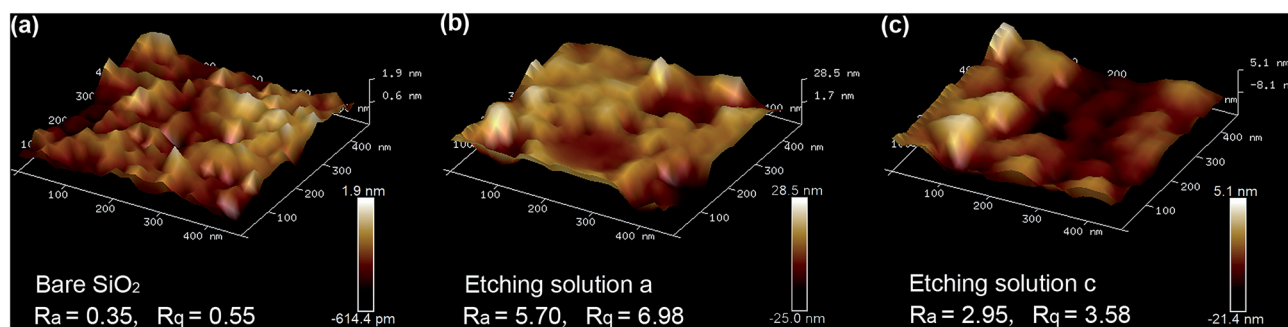
Fig. 2 AFM images of different SiO 2 chip surfaces before etching (a) and after etching by HF (b) and HF/HNO 3 (10 : 3) mixture solutions (c). Scan rate: 1 Hz. The obtained AFM data were analyzed using NanoScope Analysis 1.8, and the calculated profile roughness parameters, roughness average ( R_a ) and RMS roughness ( R_q ), were labeled in the bottom of this figure. Height ranges ( \delta h ) of each areas were calculated based on the differences from obtained height bars.
