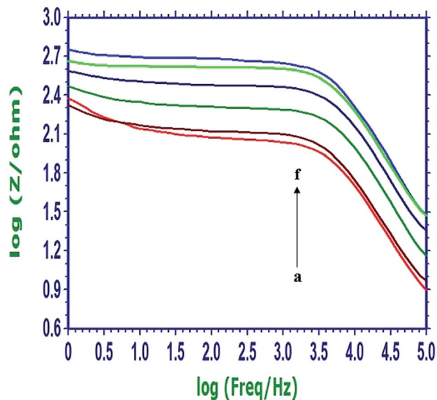
Fig. 4 Representative Bode plots of the PI6COOH/WS 2 /CPE (a), dsDNA/PI6COOH/WS 2 /CPE (hybridized with cDNA), (b), hybridized with single-base mismatched DNA (c), hybridized with three-base mismatched DNA (d), hybridized with ncDNA (e), and ssDNA/PI6COOH/WS 2 /CPE (f) in 0.3 mol L -1 PBS (pH 7.0).
