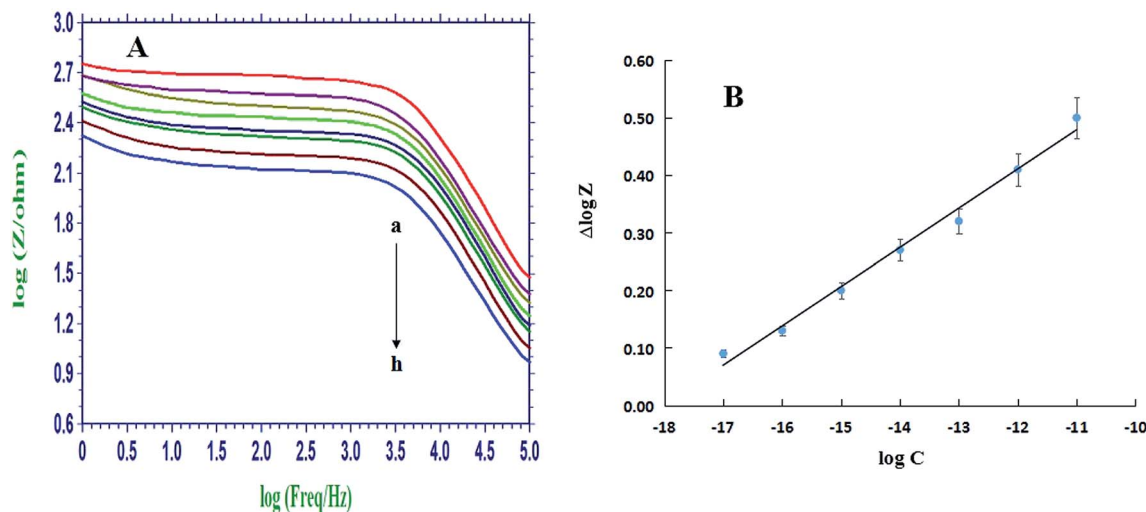
Fig. 5 (A) Representative Bode plots of the ssDNA/PI6COOH/WS 2 /CPE (a) and after hybridization reaction with different concentrations of PIK3CA gene target sequences: (b) 1.0 \times 10^{-17} , (c) 1.0 \times 10^{-16} , (d) 1.0 \times 10^{-15} , (e) 1.0 \times 10^{-14} , (f) 1.0 \times 10^{-13} , (g) 1.0 \times 10^{-12} and (h) 1.0 \times 10^{-11} mol L -1 in 0.3 mol L -1 PBS (pH 7.0). (B) The plot of \Delta \log Z versus the logarithm of the PIK3CA gene target sequence concentrations.
