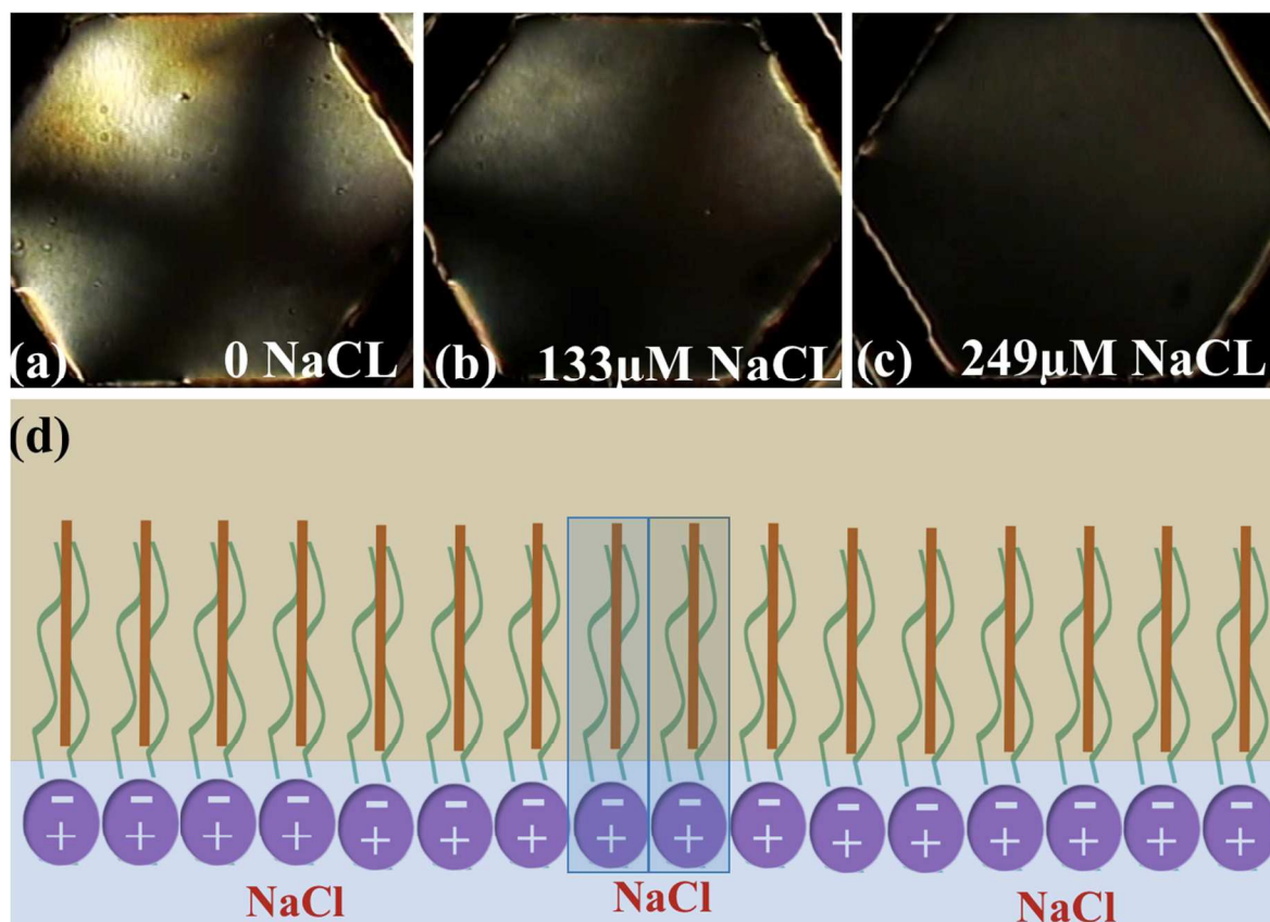
Figure 6: Illustration of the effect of added salt ( \text{NaCl} ) on the texture of the LC film at 40 \mu\text{M} DLPC concentration. (a) No \text{NaCl} added (texture is the same as shown in Figure 2(c)); (b) The texture at 133 \mu\text{M} \text{NaCl} concentration is darker, though the Maltese cross is still visible, indicating a less bent LC surface; (c) The texture at 249 \mu\text{M} \text{NaCl} concentration is completely dark indicating flat LC film surface with homeotropic alignment; (d) Cartoon of the effect of the \text{Na}^+ and \text{Cl}^- ions on the effective of the DLPC molecules.
