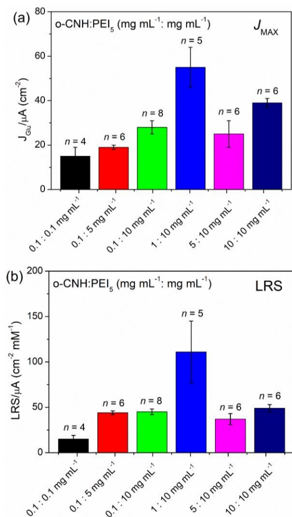
Fig. 5 Histograms depicting the increase in both the J_{\text{MAX}} and LRS of a o-CNH-PEI design as the concentration increases up to a maximum of 10 \text{mg mL}^{-1} o-CNH-PEI , after which, the J_{\text{MAX}} and LRS decline.
