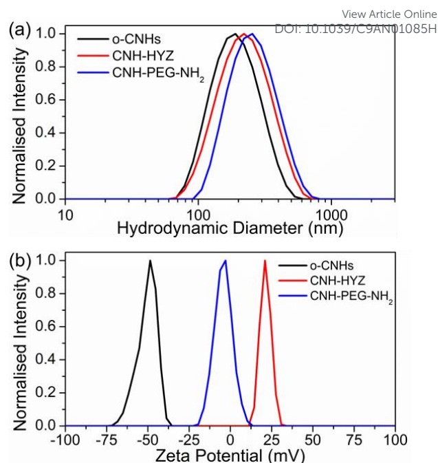
Fig. 2 (a) Dynamic light scattering (b) Zeta potential measurements of o -CNH, CNH-HYZ and CNH-PEG-NH 2 obtained in ddH 2 O, pH 7.2 at 25 °C
