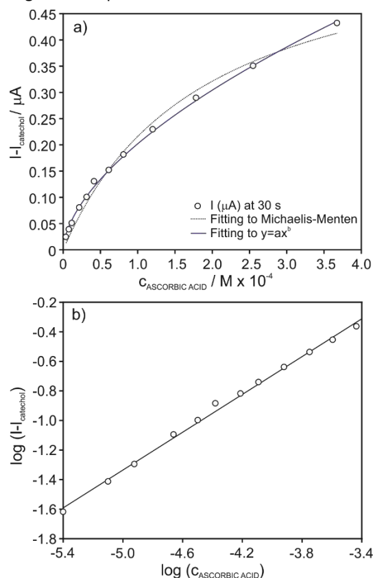
Figure 6. (a) Plot of the absolute current change for increasing concentration of ascorbic acid in the presence of 4 \times 10^{-5} M catechol concentration. (b) Calibration graph after data linearization.
