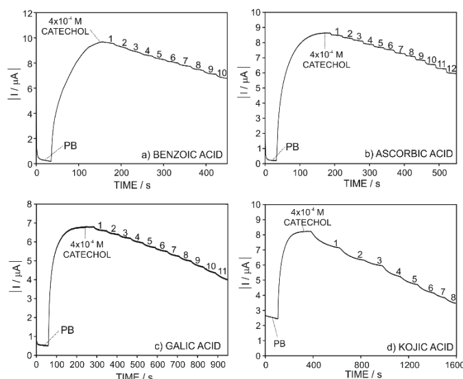
Figure 4. Dynamic response of the sensors at a fixed concentration of catechol ( 4 \times 10^{-4} M) and gradually increasing the inhibitor concentration in the solution: (a) Benzoic acid, (b) Ascorbic acid, (c) Gallic acid, (d) Kojic acid.
