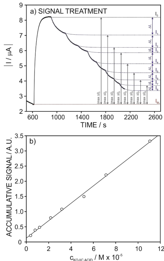
Figure 8. (a) Recorded current response for increasing kojic acid concentration (black) and the corresponding extrapolated fitted curves (dashed blue line). (b) Calibration graph observed after linearization.
