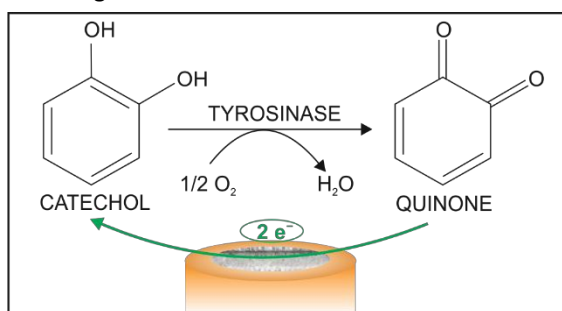
Figure 2. Illustration of the response mechanism of the biosensor.
