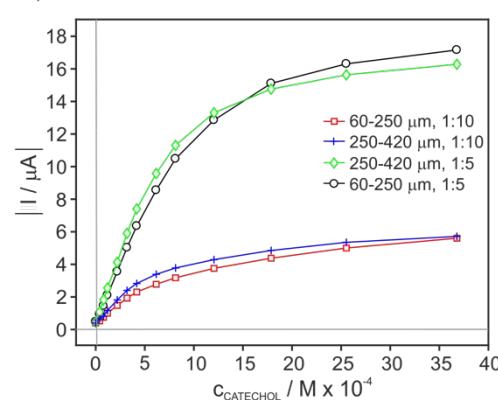
Figure 1. Influence of (a) the applied potential and (b) paste composition and particle size in the recorded current.
