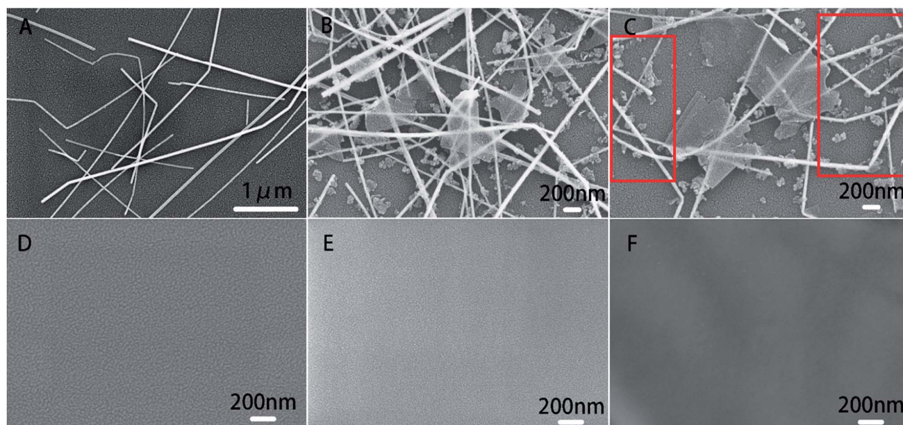
Fig. 1 SEM images of (A) AgNWs/SiO 2 , (B) and (C) Gra/AgNWs/SiO 2 , (D) \text{TiO}_2 -CS/Gra/AgNWs/SiO 2 , (E) CS/ \text{TiO}_2 -CS/Gra/AgNWs/SiO 2 and (F) AChE/CS/ \text{TiO}_2 -CS/Gra/AgNWs/SiO 2 (second electron detector). The concentration of AgNWs is 2 mg ml -1 and AChE is 5 mg ml -1 .
