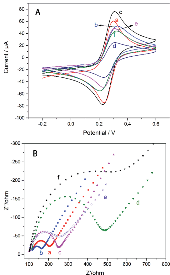
Fig. 3 (A) The CV and (B) the EIS of (a) GC, (b) AgNWs/GC, (c) Gra/AgNWs/GC, (d) \text{TiO}_2\text{-CS/Gra/AgNWs/GC} , (e) \text{CS/TiO}_2\text{-CS/Gra/AgNWs/GC} , (f) \text{AChE/CS/TiO}_2\text{-CS/Gra/AgNWs/GC} electrodes, [\text{Fe}(\text{CN})_6]^{3-/4-} (10/10 mM). AChE concentration: 5 \text{ mg ml}^{-1} .
