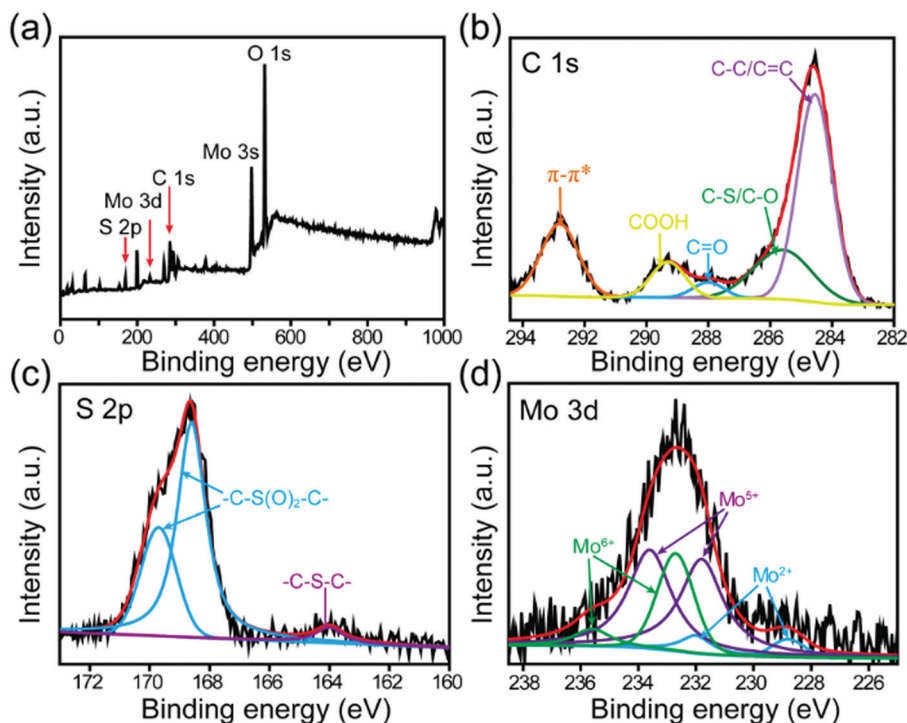
Fig. 2 (a) XPS spectra of Mo-CQDs. (b, c and d) High resolution XPS spectra of C 1s, S 2p and Mo 3d.
