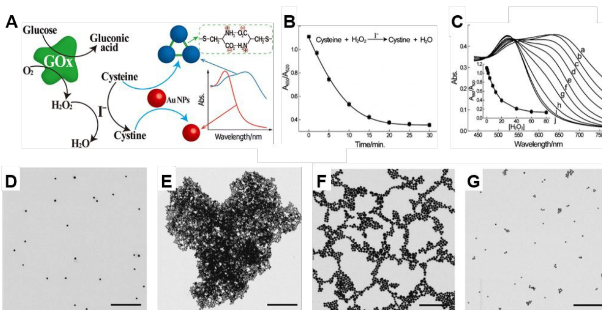
Figure 8. Reversible colorimetric sensor based on nanoparticle aggregation. (A) Schematic representation of oxidation-induced nanoparticle interactions and resulting absorbance shifts mediated through cysteine/cystine transformations (B) Characteristic time-dependent change in absorbance ratio of un-aggregated AuNPs (520 nm) to aggregated AuNPs (650nm) as a result of the iodide ( I^- ) catalyzed oxidation of cysteine by H_2O_2 (20 \mu M ) over 30 minutes (C) Absorbance shifts as a result of cysteine capped AuNPs treated with differing concentrations of H_2O_2 (a-j) corresponding to a range of 0-80 \mu M . I^- concentration was fixed at 2 \mu M . Inset is a calibration curve derived from the absorbance of the aggregated AuNPs and H_2O_2 concentration, demonstrating aggregation inhibition as H_2O_2 concentration increases. Analysis indicated a detection limit of 2 \mu M H_2O_2 (D-G) TEM images of AuNP aggregates resulting from treatment with H_2O_2 . (D = bare AuNPs; E = no H_2O_2 ; F = 16 \mu M of H_2O_2 + 0.2 \mu M I^- ; G = 40 \mu M H_2O_2 + 0.2 \mu M I^- . Reprinted with permission from ref. 86. Copyright 2013 American Chemical Society.
