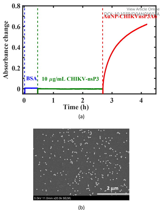
Figure 4. (a) Temporal response showing binding kinetics of AuNP-CHIKVnsP3Ab on U-bent fiber surface exposed to 10 \mu\text{g/mL} CHIKV-nsP3 obtained using LED-PD set-up. (b) HR-SEM image of a U-bent POF probe showing the AuNP labels.
