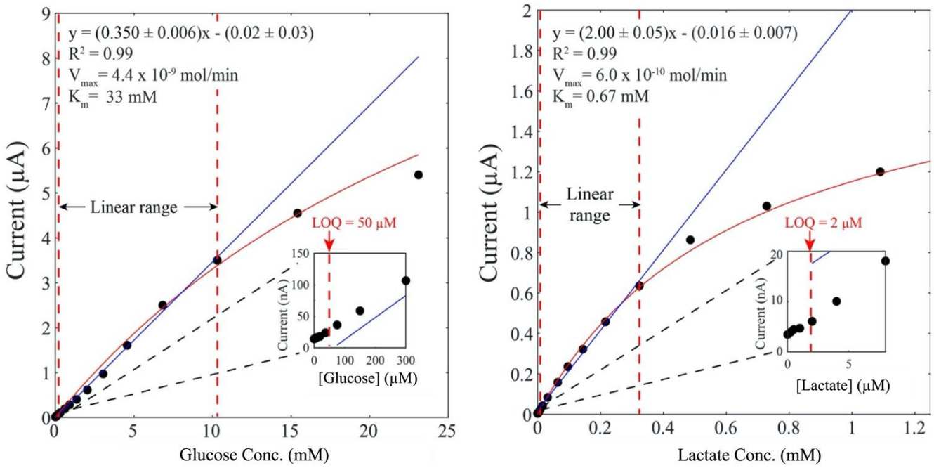
Figure 2. Representative calibration curves of anodic current vs. analyte concentration showing the limits of linearity, limits of quantitation, V_{max} , and K_m for Os-based GOx (left) and LOx (right) sensors. The linear range, indicated by the two dotted red lines, were 50 μM to 10 mM and 2 to 324 μM for glucose and lactate, respectively. The slopes are represented by solid blue lines [ y = (0.350 \pm 0.006)x - (0.02 \pm 0.03) , R^2 = 0.99 ] for the Os-polymer GOx sensor and [ y = (2.00 \pm 0.05)x - (0.016 \pm 0.007) , R^2 = 0.99 ] for the Os-based LOx sensor. Using non-linear regression, shown in solid red, V_{max} and K_m were calculated for both analytes. For the Os-based GOx sensor, V_{max} was 4.4 \times 10^{-9} \text{ mol min}^{-1} and K_m was 33 mM. The Os-polymer LOx had a V_{max} of 6.0 \times 10^{-10} \text{ mol min}^{-1} and K_m of 0.67 mM. Inset: zoom-in of the lower concentrations of each analyte showing the lower limit of linearity (limit of quantitation). Experiments were performed in buffered saline solution (ambient conditions).
