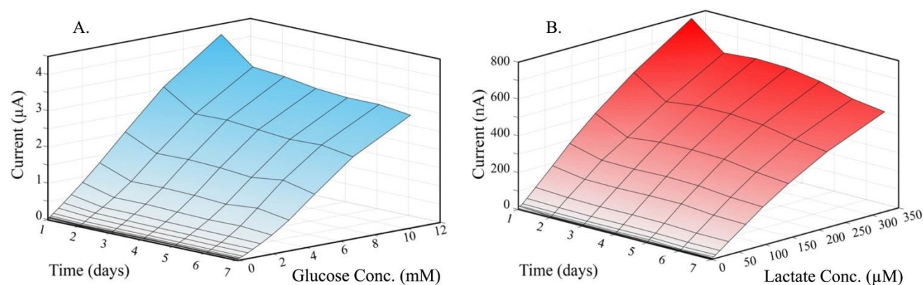
Figure 3. Operational longevity of the Os-based GOx (A) and LOx (B) sensors was tested by calibrating daily for seven days. Anodic (oxidative) current vs. calibration day vs. analyte concentration reported above. The sensitivity of the GOx sensor decreased from 420 \pm 7 \text{ nA mM}^{-1} to 313 \pm 7 \text{ nA mM}^{-1} , and the LOx sensor sensitivity decreased from 2460 \pm 70 \text{ nA mM}^{-1} to 1730 \pm 70 \text{ nA mM}^{-1} in the course of the week. Experiments were performed in buffered saline solution (ambient conditions) at 0.2 V. Data represented as the average, n = 3 replicates.
