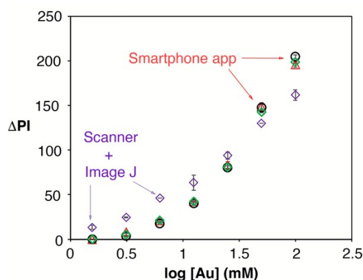
Figure 6. Calibration plot obtained by evaluating the colorimetric signal generated by gold nanoparticles at different concentrations with the densitometry app when the room illuminance was 200 (black dots), 570 (green diamonds) and 1070 lux (red triangles), or with a desktop scanner (purple diamonds); Error bars are the standard deviation ( n = 3 ).
