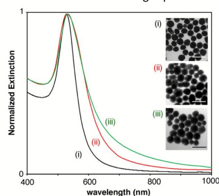
Figure 2. Extinction spectra and representative TEM images of the (i) PVP-coated, (ii) carboxylate-coated, and (iii) amine-coated nanoparticles used as starting materials for developing colorimetric nanoprobes. Scale bars: 100 nm.
