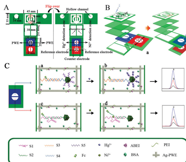
Fig. 26 An electrochemiluminescence paper device for the detection of Hg 2+ and Ni 2+ . Reprinted (adapted) with permission from Y. Huang, L. Li, Y. Zhang, L. Zhang, S. Ge and J. Yu, Auto-cleaning paper-based electrochemiluminescence biosensor coupled with binary catalysis of cubic Cu 2 O–Au and polyethyleneimine for quantification of Ni 2+ and Hg 2+ , Biosens. Bioelectron. , 2019, 126 , 339–345. Copyright 2018 Elsevier B.V. 133
