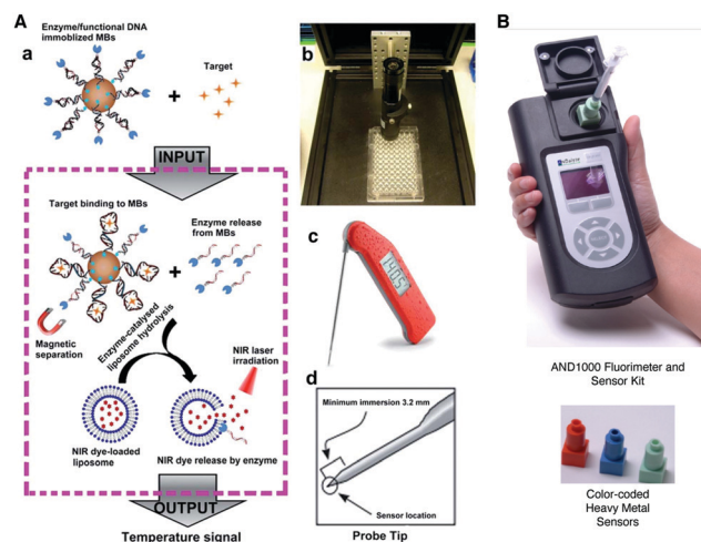
Fig. 21 (A) Detection of target analyte using a smart thermometer. Reprinted (adapted) with permission from J. Zhang, H. Xing and Y. Lu, Translating molecular detections into a simple temperature test using a target-responsive smart thermometer, Chem. Sci. , 2018, 9 , 3906–3910. Copyright 2018, The Royal Society of Chemistry. 301 (B) ANDalyze Portable Fluorescence Reader and disposable sensors. Copyright permission granted by ANDalyze.
