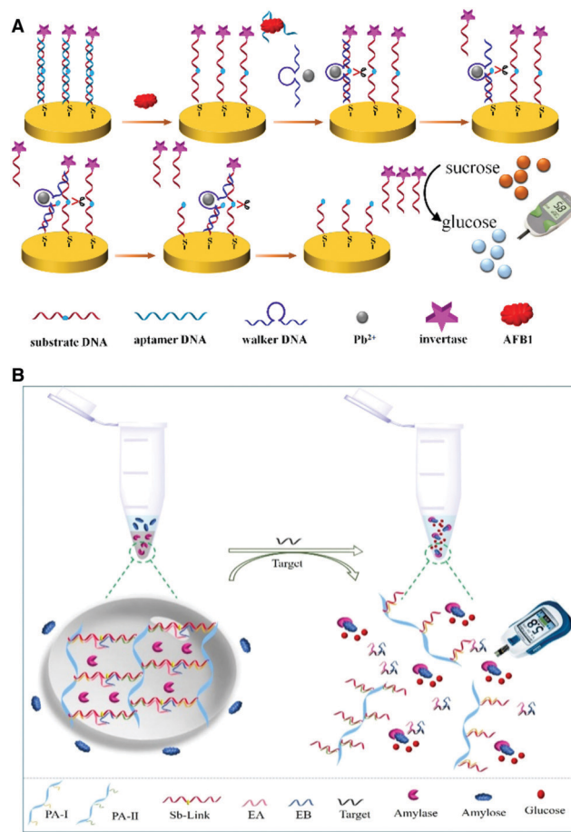
Fig. 23 DNzyme based devices for the detection of non-metal targets. (A) A PGM-sensor for the detection of aflatoxin B1. Reprinted (adapted) from X. Yang, D. Shi, S. Zhu, B. Wang, X. Zhang and G. Wang, Portable Aptasensor of Aflatoxin B1 in Bread Based on a Personal Glucose Meter and DNA Walking Machine, ACS Sens. , 2018, 3 , 1368–1375. Copyright 2018, American Chemical Society. 316 (B) Detection of microRNAs by PGM and oligonucleotide cross-linked hydrogel. Reprinted (adapted) from Y. Si, L. Li, N. Wang, J. Zheng, R. Yang and J. Li, Oligonucleotide Cross-Linked Hydrogel for Recognition and Quantitation of MicroRNAs Based on a Portable Glucometer Readout, ACS Appl. Mater. Interfaces , 2019, 11 , 7792–7799. Copyright 2019, American Chemical Society. 317
