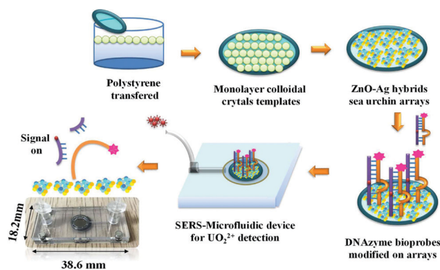
Fig. 20 Schematic representation of the detection of uranyl ion using a microfluidic SERS device. Reprinted (adapted) from X. He, X. Zhou, Y. Liu and X. Wang, Ultrasensitive, recyclable and portable microfluidic surface-enhanced Raman scattering (SERS) biosensor for uranyl ions detection, Sens. Actuators, B , 2020, 311 , 127676, with permission from Elsevier. 300
