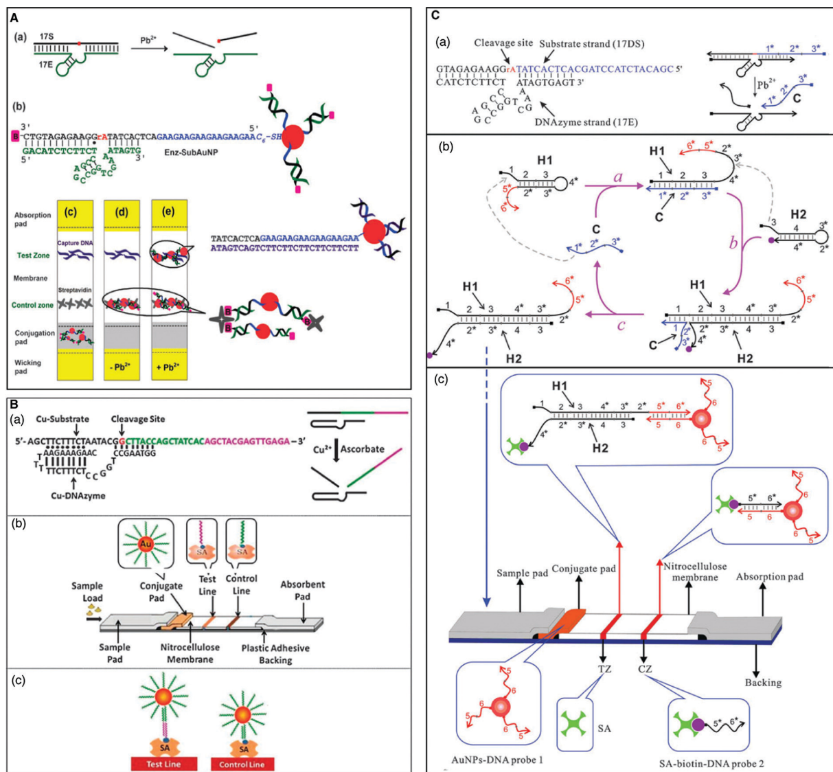
Fig. 24 DNAzyme based lateral flow devices (LFDs). (A) An LFD for the detection of Pb 2+ using 8–17 DNAzyme. Reprinted (adapted) from D. Mazumdar, J. Liu, G. Lu, J. Zhou, Y. Lu, Easy-to-use dipstick tests for detection of lead in paints using non-cross-linked gold nanoparticle–DNAzyme conjugates, Chem. Commun. , 2010, 46 , 1416–1418, with permission from The Royal Society of Chemistry. 43 (B) LFD-based Detection of Cu 2+ using Cu–DNAzyme. Reprinted (adapted) from Z. Fang, J. Huang, P. Lie, Z. Xiao, C. Ouyang, Q. Wu, G. Liu, L. Zeng, Lateral flow nucleic acid biosensor for Cu 2+ detection in aqueous solution with high sensitivity and selectivity, Chem. Commun. , 2010, 46 , 9043–9045, with permission from The Royal Society of Chemistry. 321 (C) A biosensor for Pb 2+ detection using 8–17 DNAzyme and catalytic hairpin assembly. Reprinted (adapted) from J. Chen, X. Zhou, L. Zeng, Enzyme-free strip biosensor for amplified detection of Pb 2+ based on a catalytic DNA circuit, Chem. Commun. , 2013, 49 , 984–986, with permission from The Royal Society of Chemistry. 322
