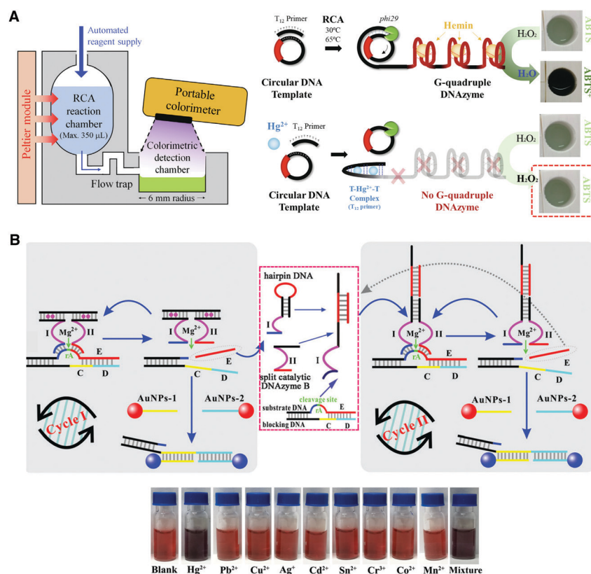
Fig. 19 Portable colorimetric devices for the detection of mercury. (A) Schematic representation of the sensing strategy for a 3D-printed rolling circle amplification chip for on-site colorimetric detection of mercury. Reprinted (adapted) from J. W. Lim, T.-Y. Kim, S.-W. Choi and M.-A. Woo, 3D-printed rolling circle amplification chip for on-site colorimetric detection of inorganic mercury in drinking water, Food Chem. , 2019, 300 , 125177, with permission from Elsevier. 265 (B) Naked-eye colorimetric detection of \text{Hg}^{2+} using an AuNP assay. Reprinted (adapted) from J. Chen, J. Pan and S. Chen, A naked-eye colorimetric sensor for \text{Hg}^{2+} monitoring with cascade signal amplification based on target-induced conjunction of split DNzyme fragments, Chem. Commun. , 2017, 53 , 10224–10227, with permission from The Royal Society of Chemistry. 142
