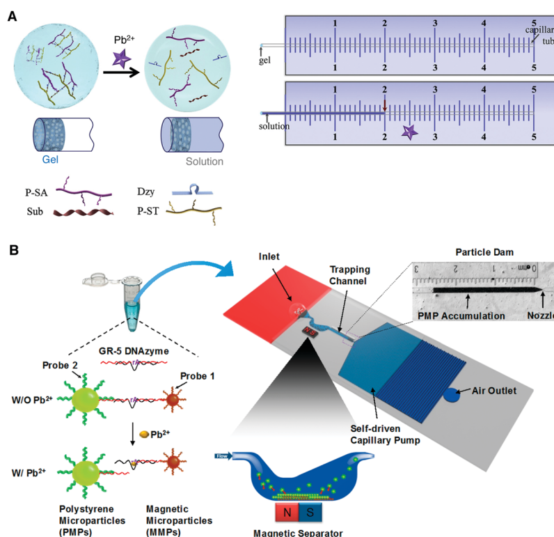
Fig. 18 Portable DNAzyme devices for the detection of \text{Pb}^{2+} based on visual reading of capillary flow. (A) A portable hydrogel capillary sensor. Reprinted (adapted) from C. Jiang, Y. Li, H. Wang, D. Chen and Y. Wen, A portable visual capillary sensor based on functional DNA crosslinked hydrogel for point-of-care detection of lead ion, Sens. Actuators, B , 2020, 307 , 127625, with permission from Elsevier. 177 (B) A portable sensor with a microfluidic particle dam. Reprinted (adapted) with permission from G. Wang, L. T. Chu, H. Hartanto, W. B. Utomo, R. A. Pravasta and T.-H. Chen, Microfluidic Particle Dam for Visual and Quantitative Detection of Lead Ions, ACS Sens. , 2020, 5 , 19–23. Copyright 2020, American Chemical Society. 178
