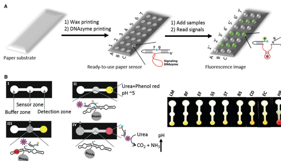
Fig. 28 DNAzyme based paper sensors for bacterial detection. (A) Paper plate sensor for bacterial detection. Reprinted (adapted) with permission from M. M. Ali, C. L. Brown, S. Jahanshahi-Anbuhi, B. Kannan, Y. Li, C. D. M. Filipe and J. D. Brennan, A Printed Multicomponent Paper Sensor for Bacterial Detection, Sci. Rep. , 2017, 7 , 12335. Copyright 2017 Ali et al. 47 (B) A colorimetric paper-based sensor using the HP DNAzyme and a modified version of the urease-based litmus test for the detection of H. pylori . HP: H. pylori ; others are control bacteria. Reprinted (adapted) with permission from M. M. Ali, M. Wolfe, K. Tram, J. Gu, C. D. M. M. Filipe, Y. Li and J. D. Brennan, A DNAzyme-Based Colorimetric Paper Sensor for Helicobacter pylori , Angew. Chem., Int. Ed. , 2019, 1 , 9907–9911. Copyright 2019 Wiley-VCH Verlag GmbH & Co. KGaA, Weinheim. 48
