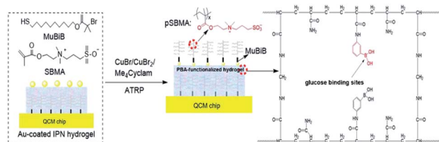
Fig. 1 Schematic diagram showing the synthesis procedure for the HFSA. (b) An HFSA-coated quartz chip (i). An SEM image of the cross-sectional HFSA (ii). A schematic diagram illustrating the protein resistance and glucose sensitivity of the HFSA (iii). (c) The traditional anti-fouling coating modified hydrogel film has poor glucose sensitivity.
