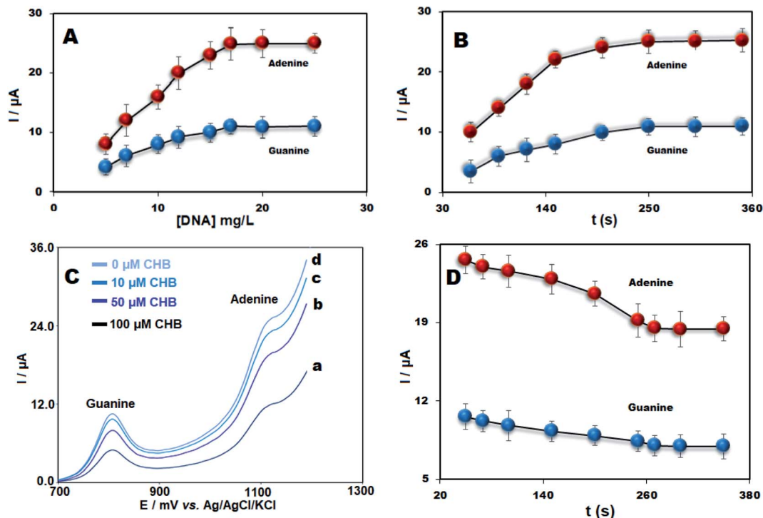
Fig. 4 (A) The plot of oxidation signal of adenine and guanine vs. diverse ds-DNA concentrations ( 5\text{--}25\text{ mg L}^{-1} ) and (B) various accumulation time. (C) DPV for ds-DNA/PPy/FL-Pt/ \text{NiCo}_2\text{O}_4 /PGE in the presence of (a) 0, (b) 10, (c) 50 and (d) 100 \mu\text{M} CHB and (D) The incubation time effect of 50.0 \mu\text{M} CHB on the response of ds-DNA/PPy/FL-Pt/ \text{NiCo}_2\text{O}_4 /PGE ( n = 3 ).
