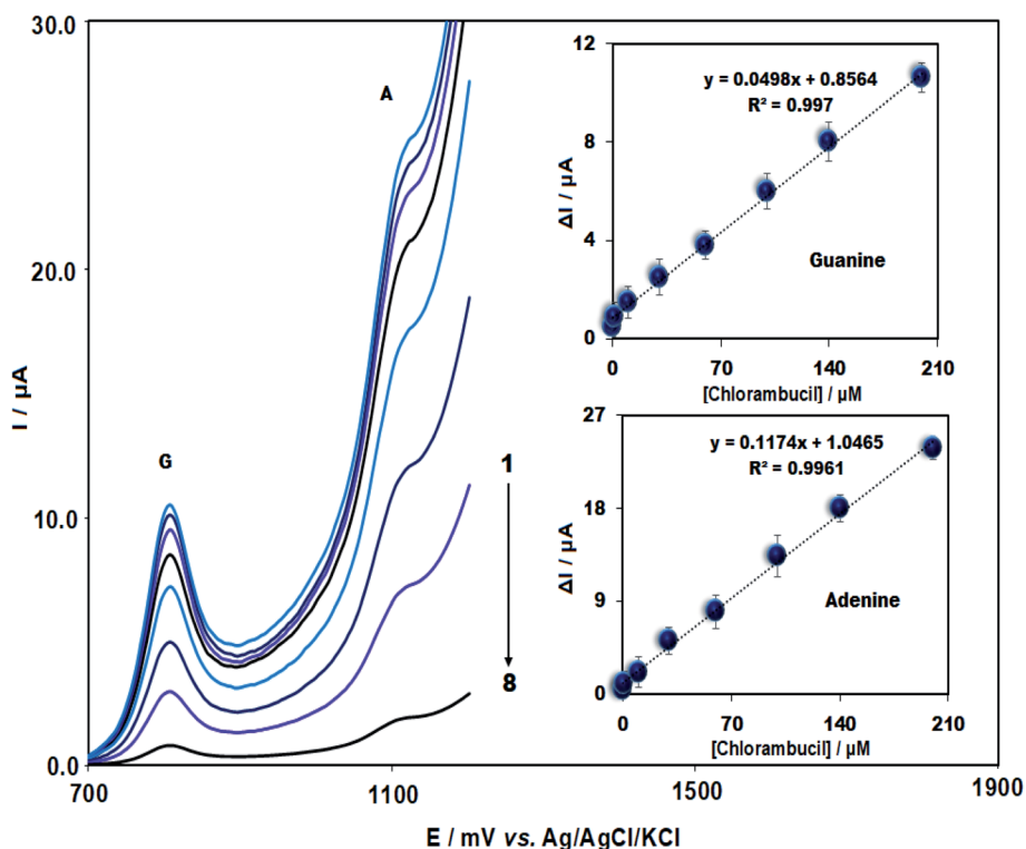
Fig. 5 DPV voltammograms for different CHB concentrations in 0.5 M ABS ( \text{pH} = 4.8 ) at ds-DNA/PPy/FL-Pt/ \text{NiCo}_2\text{O}_4 /PGE. From top to bottom: 0.018, 1.0, 10.0, 30.0, 60.0, 100.0, 140.0 and 200.0 \mu\text{M} ; insets: the net current of adenine and guanine versus concentrations of CHB ( n = 3 ).
