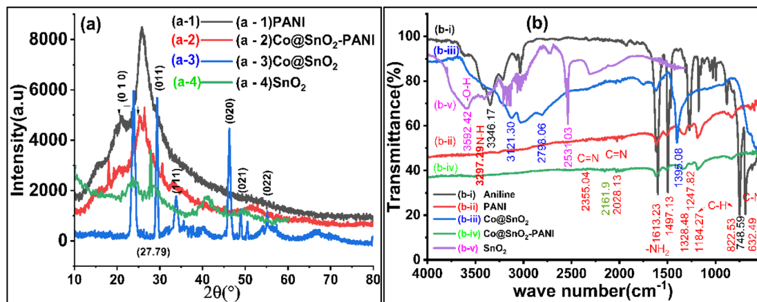
Fig. 1 (a) XRD data plots of (a-4) \text{SnO}_2 , (a-1) PANI, (a-3) \text{Co@SnO}_2 , and (a-2) \text{Co@SnO}_2 -PANI (b) FTIR plots of (b-i) aniline, (b-ii) PANI, (b-iii) \text{Co@SnO}_2 , and (b-iv) \text{Co@SnO}_2 -PANI.
