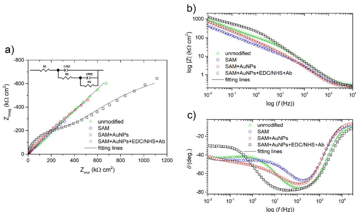
Fig. 3 Nyquist (a) and Bode (b and c) representations of the impedance spectra recorded for unmodified and modified gold electrodes at E_{\text{OC}} after 30 min of exposure in a solution of 0.1 M \text{KNO}_3 with 5 mM [\text{Fe}(\text{CN})_6]^{3-/4-} . Solid fitting lines refer to Model 2 from Fig. 4b.
