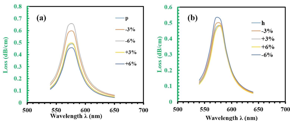
Fig. 7 (a) Pitch tolerance on the confinement loss of RI 1.34 with in \pm 6\% . (b) Channel distance tolerance from center of the plasmonic layer.
