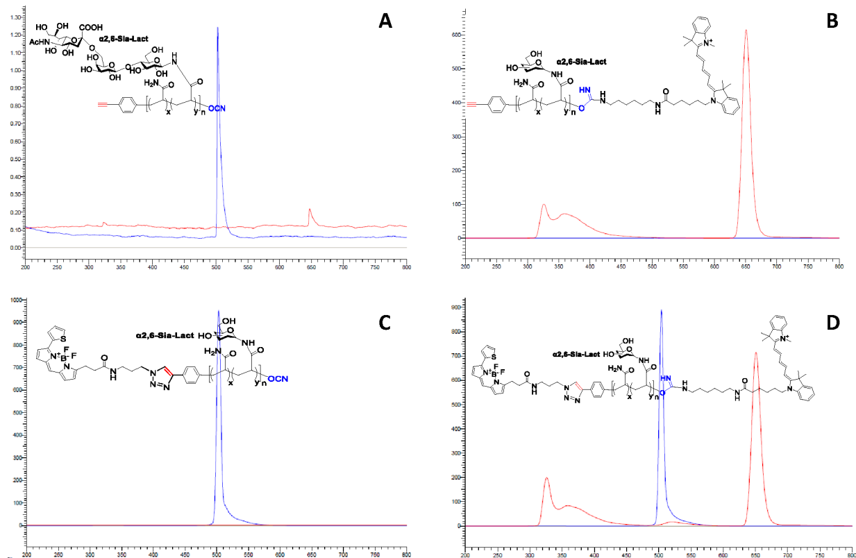
Figure 3. Fluorescent emission spectra of chain-end functionalized alkyne- \alpha 2,6-Sia-Lact glycopolymer. (A) Alkyne- \alpha 2,6-Sia-Lact glycopolymer, (B) Alkyne- \alpha 2,6-Sia-Lact-Cy5 glycopolymer, (C) Bodipy- \alpha 2,6-Sia-Lact glycopolymer, (D) Bodipy- \alpha 2,6-Sia-Lact-Cy5 glycopolymer (Red excitation wavelength 646 nm, blue excitation wavelength 502 nm in H 2 O).
