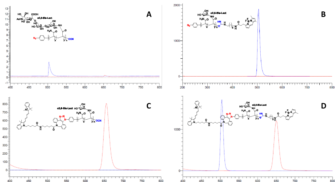
Figure 5. Fluorescent emission spectra of chain-end functionalized \alpha 2,6 -Sia-Lact glycopolymers. (A) Azide- \alpha 2,6 -Sia-Lact glycopolymer, (B) Azide- \alpha 2,6 -Sia-Lact-Bodipy glycopolymer, (C) Cy5- \alpha 2,6 -Sia-Lact glycopolymer, (D) Cy5- \alpha 2,6 -Sia-Lact-Bodipy glycopolymer (Red excitation wavelength 646 nm, blue excitation wavelength 502 nm in H_2O ).
