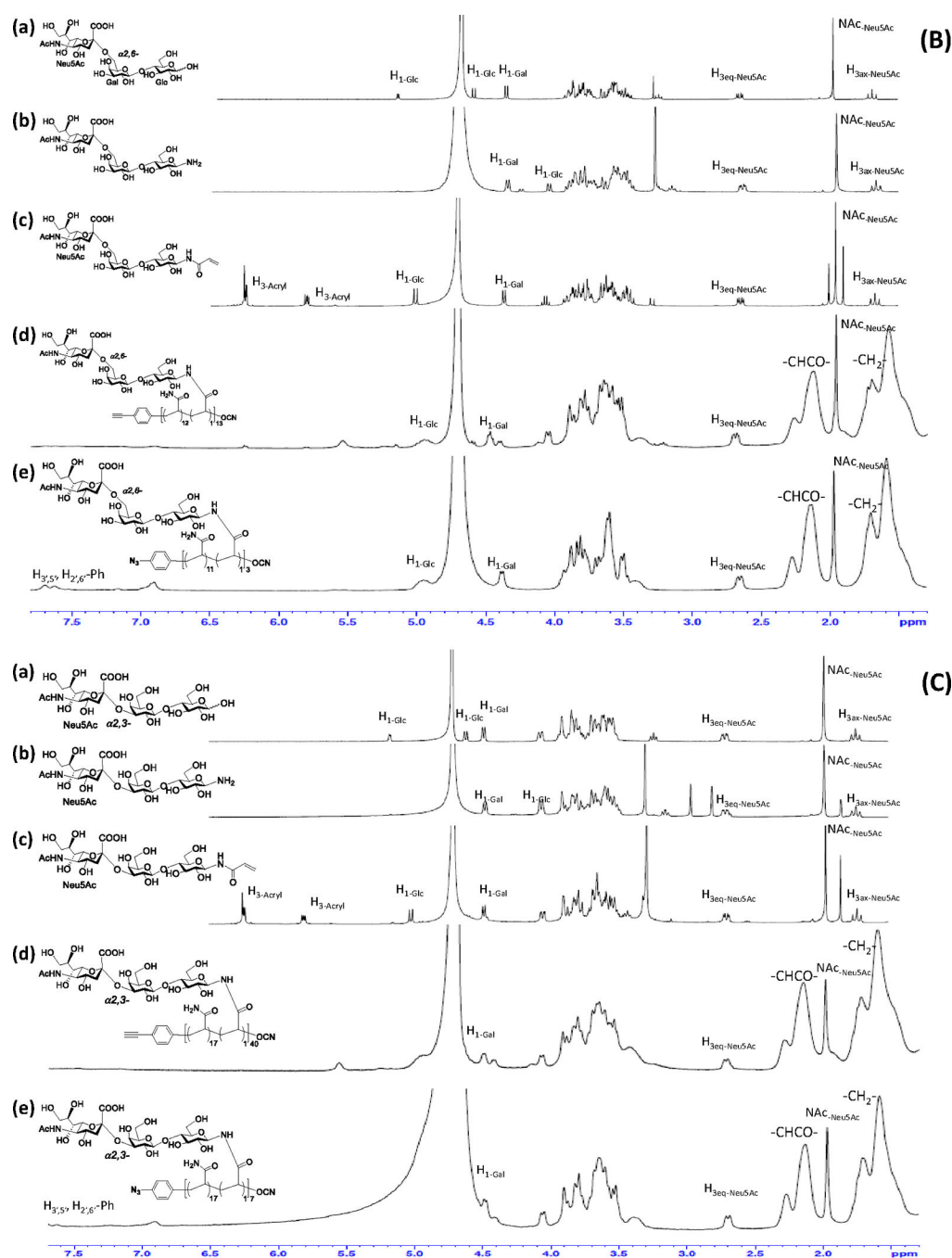
Figure 1. ^1\text{H} NMR spectra of \alpha,\omega -end orthogonally functionalizable glycopolymers.
