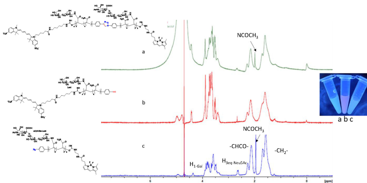
Figure 6. ^1\text{H} NMR spectra and photo images under UV light of a) \alpha 2,6-Sia-Lact-Bodipy and Lact glycopolymer-Cy5 dimer, b) Alkyne-Lact glycopolymer-Cy5, c) Azide- \alpha 2,6-Sia-Lact-Bodipy glycopolymer (400 MHz, \text{D}_2\text{O} ).
