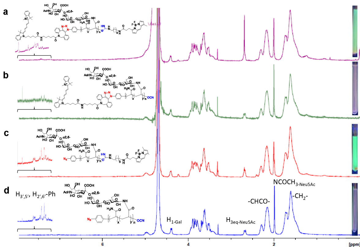
Figure 4. ^1\text{H} NMR spectra and photo images under UV light of chain-end functionalized \alpha 2,6 -Sia-Lact glycopolymers.
