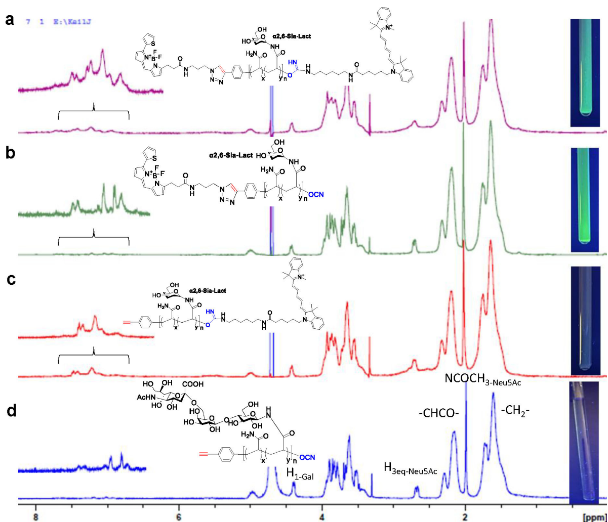
Figure 2. ^1\text{H} NMR Spectra and photo images under UV light of chain-end functionalized alkyne- \alpha 2,6-Sia-Lact glycopolymers.
