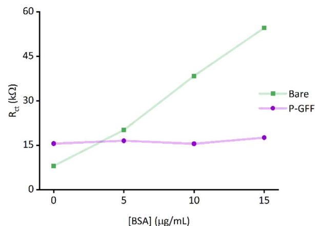
Fig. 7 Extracted R_{\text{ct}} parameters for BSA incubation of both bare and P-GFF modified Au-SPEs.
