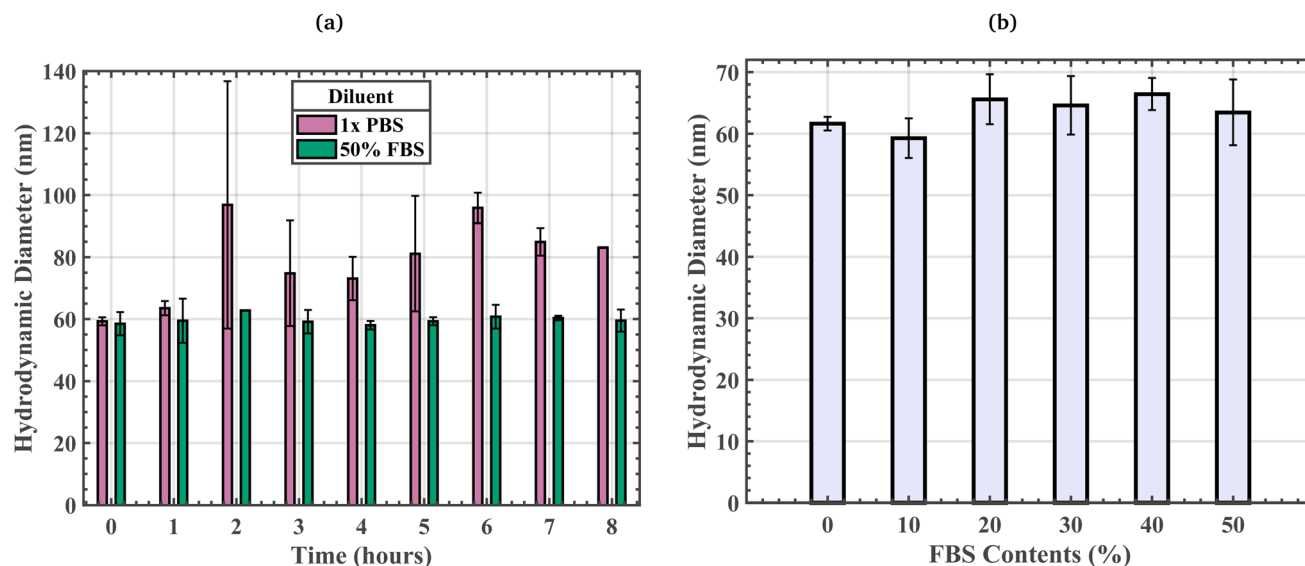
Fig. 6 (a) Time evolution of biotin-PEG 4 -MNP D_{\text{Hvd}} while suspended in 1× PBS and 50% FBS at room temperature. These data suggest that the presence of the off-target serum proteins present in 50% FBS stabilized our biotin-PEG 4 -MNPs against aggregation for at least 8 hours. The error bars represent an 80% confidence interval on each mean value. (b) Biotin-PEG 4 -MNP D_{\text{Hvd}} in 0% (1× PBS), 10%, 20%, 30%, 40%, and 50% FBS solutions. The error bars represent a 95% confidence interval on each mean value.
