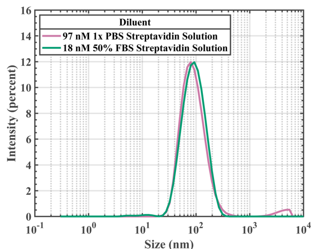
Fig. 2 Biotin-PEG 4 -MNP D_{\text{Hyd}} while suspended in a 97 nM 1× PBS streptavidin solution was indistinguishable from biotin-PEG 4 -MNP D_{\text{Hyd}} while suspended in a 18 nM 50% FBS streptavidin solution. These data suggest that the off-target serum proteins present in 50% FBS increased biotin-PEG 4 -MNP streptavidin sensitivity.
