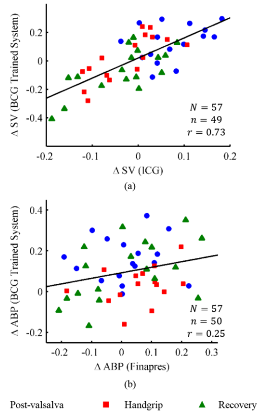
FIGURE 5. (a) Correlation results for stroke volume values obtained from the BCG mapped waveforms and the ICG waveforms. The relationship is statistically significant ( p < 0.05 ) (b) Correlation results for change in pulse pressure from the BCG mapped and original ABP waveforms. N represents the total number of data points while n denotes the number of data points considered in the analysis after outlier rejection.
