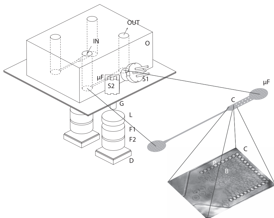
FIG. 1. PDMS block with the tubing (IN, OUT), illumination (S1, S2), detection (D), microfluidic channel ( \mu F ), and cage (C) to trap agarose beads (B) filled with bacteria. For description of the other components, see the main text.
