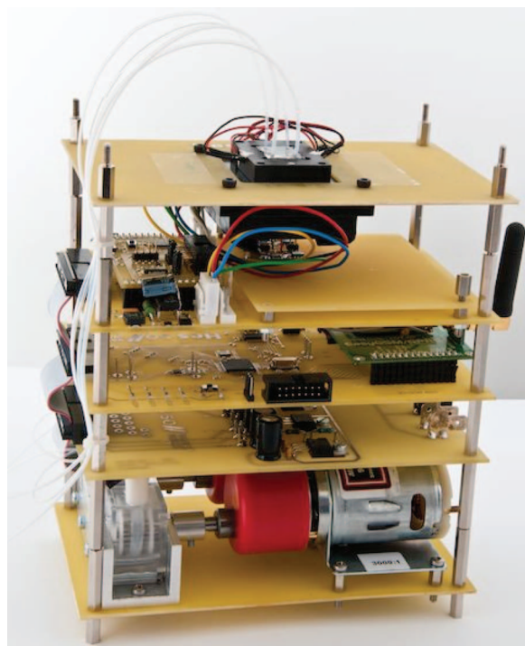
FIG. 2. The overall biosensor device with the microfluidic cell chip on top ( 10 \times 16 \times 25 \text{ cm}^3 ). The device uses a 12 V power supply and communicates via GSM or via USB with a computer.
