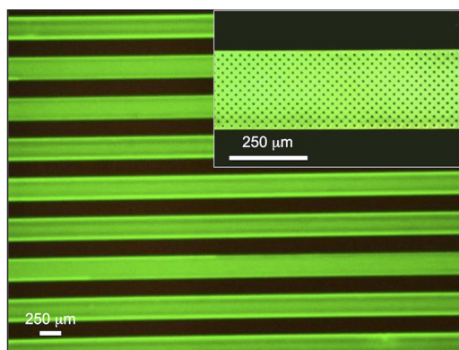
FIG. 1. Fluorescence image (AF488) of MBD-biotin attachment to the SiO 2 surface of the microfluidic channel. Inset shows a magnified view of the microfluidic channel.
