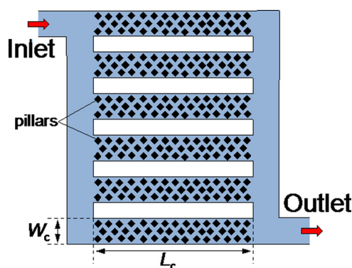
FIG. 2. Schematic diagram of the microchannels of the \mu SPE LOC system.
