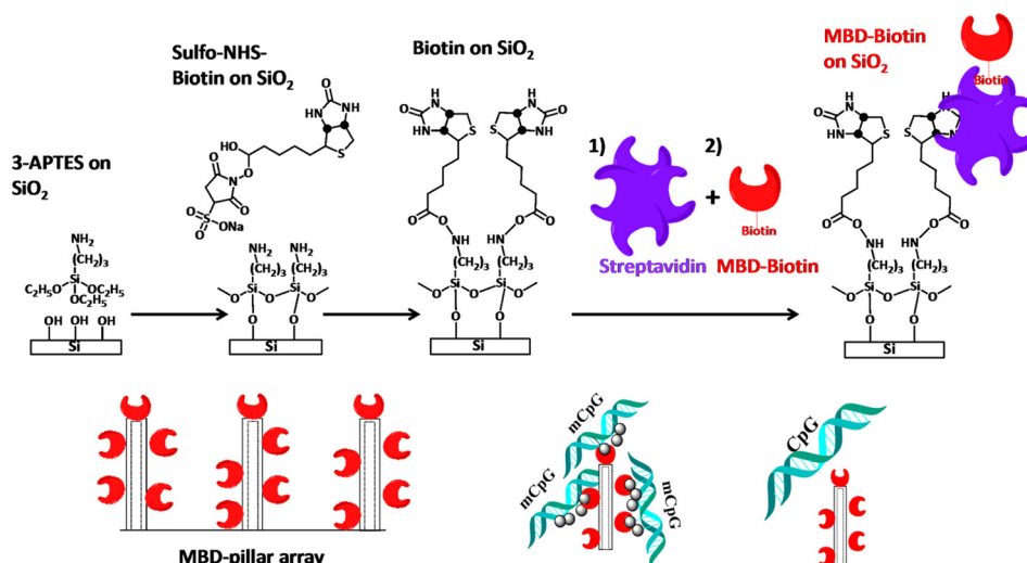
SCHEME 1. Surface functionalization of MBD-biotin proteins to the SiO 2 surface of the microchannel.
