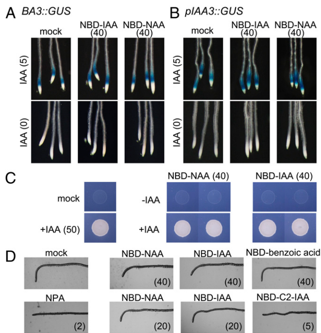
Fig. 2. Effects of NBD-auxins on SCFTIR1 auxin signaling. (A and B) Effects of NBD-auxins on auxin-responsive reporter gene expression. Six-day-old BA3::GUS (A) and pIAA3::GUS (B) lines were incubated with or without IAA, together with NBD-auxins, for 5 h or 16 h, respectively. (C) Yeast two-hybrid assay in which TIR1-DBD and Aux/IAA(IAA7)-AD fusion proteins were expressed. IAA enhanced the interaction between TIR1 and Aux/IAA to rescue LEU2 -deficient yeast growth. (D) Effect of NBD-labeled analogs on the root gravitropic response. Roots (6-d-old) were placed on GM agar plates containing chemicals and grown in the dark for 5 h after rotating the plates at a 90° angle against the vertical direction. The values in parentheses indicate the concentrations of chemicals ( \mu M).
