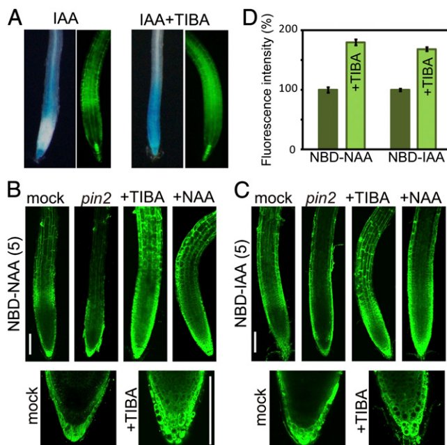
Fig. 3. Auxin transport system affects the distribution of fluorescent auxin in roots. (A) Effects of auxin transport inhibitors on the auxin-responsive DR5 expression profile. Six-day-old DR5::GUS (Left) and DR5::GFP (Right) lines were treated with or without 20 \mu M TIBA, together with 2 \mu M IAA, for 5 h or 8 h, respectively. (B and C) Wild type (Columbia-0) and pin2leir1-1 mutants were treated with 5 \mu M NBD-auxins for 15 min. Wild-type roots were preincubated with 20 \mu M TIBA or 50 \mu M NAA for 4 h and 30 min, respectively, and then treated with 5 \mu M NBD-auxins, together with TIBA and NAA, for 15 min. The values presented in parentheses indicate the concentration of chemicals ( \mu M). (Scale bars, 100 \mu m.) (D) Arabidopsis MM1 cells were incubated with 2 \mu M NBD-auxins with or without 50 \mu M TIBA for 30 min after preincubation with TIBA for 3 h. NBD-auxins were extracted from the harvested cells using methanol and quantified with a fluorometer. Error bars represent SEM; n = 6 .
