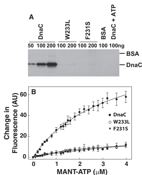
FIGURE 5. F231S and W233L are impaired in ATP-binding. A, duplicate samples of wild type DnaC, F231S, or W233L at the indicated amounts were incubated with [ \alpha - ^{32}\text{P} ]ATP (10 \mu\text{Ci} , 0.17 \mu\text{M} per reaction) for 2 min at 30 °C and then irradiated with UV light for 15 min on ice as described (10, 13). As negative controls, BSA was used in place of DnaC or DnaC was incubated in the presence of both [ \alpha - ^{32}\text{P} ]ATP and 0.1 mM ATP. One of each pair of samples was then analyzed on separate 15% SDS-polyacrylamide gels. After staining the gels with Coomassie Brilliant Blue to determine the electrophoretic positions of DnaC and BSA, autoradiography of the dried gel was performed. Because the autoradiograms of each gel were essentially identical, only one is shown. Similar results to those presented were obtained in three essentially identical experiments. B, reactions (200 \mu\text{l} ) containing 1.5 \mu\text{M} DnaC, F231S, or W233L and the indicated concentrations of MANT-ATP were incubated at 25 °C as described under "Experimental Procedures." After excitation at 356 nm, emission from 400 to 550 nm revealed an emission maximum at 440 nm. The average change in fluorescence at 440 nm and standard error from three independent measurements were plotted versus the concentration of MANT-ATP. With the mutants, almost no binding was observed.
