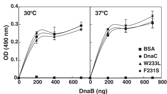
FIGURE 3. F231S and W233L are able to interact with DnaB. Enzyme-linked immunosorbent assays were performed essentially as described (20) with wild type DnaC, F231S, or W233L (200 ng in 100 \mu l of a buffer containing 10 mM \text{Na}_2\text{HPO}_4 , 1.76 mM \text{KH}_2\text{PO}_4 , 2.7 mM KCl, and 0.137 M NaCl) added per well of a microtiter plate. After incubation at room temperature for 1 h, unbound protein was removed. The indicated amounts of DnaB in triplicate were then added to each well in buffer (100 \mu l) containing 40 mM HEPES-KOH, pH 8.0, 20 mM Tris-HCl, pH 7.6, 10 mM \text{MgCl}_2 , 4 mM DTT, 1 mM ATP, and 0.1 mg/ml of BSA. After incubation for 1 h at 30 °C or 37 °C, the wells were washed with the same buffer containing 2% nonfat milk. A dilution of affinity-purified antibody that specifically recognizes DnaB was then added to each well followed by incubation at 4 °C overnight. After washing the plate as above, goat anti-rabbit antibody conjugated to horseradish peroxidase (ThermoScientific) was added, and immune complexes were detected colorimetrically at 490 nm. The average and standard deviation have been plotted.
