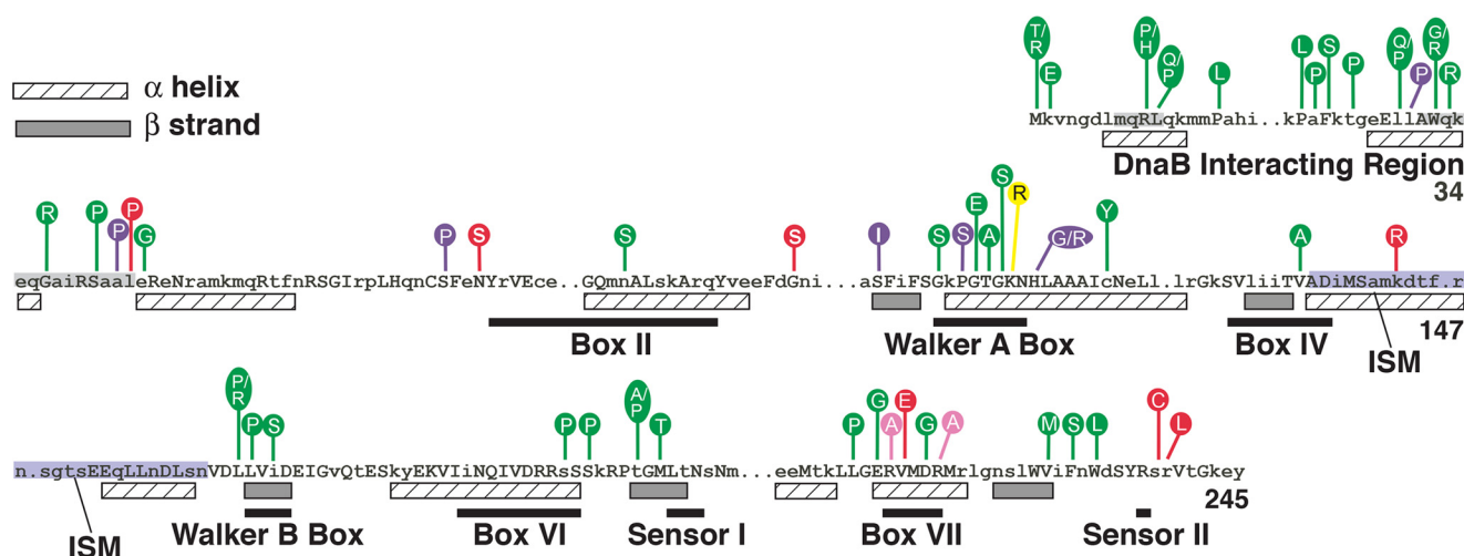
FIGURE 1. Mutant DnaC proteins and their amino acid substitutions. Alignment of the primary amino acid sequence of E. coli DnaC with 29 DnaC homologues reveals conserved residues shown as uppercase letters relative to its secondary structure ( hatched boxes , \alpha helix; filled boxes , \beta strand) derived from the A. aeolicus DnaC x-ray crystallographic structure and from a secondary structure prediction method (PHDsec) (10, 12, 14). The numbers at the right are the coordinates for E. coli DnaC protein. The figure also shows the locations of single amino acid substitutions in mutant DnaCs. Those in green are from this work; substitutions in purple , yellow , pink , and red have been described in the respective publications (10, 11, 13, 17). AAA+ motifs shown as black bars are adapted from figures in Refs. 11 and 17. The residues shaded in gray represent segments that bind to DnaB (28). Those shaded in blue correspond to the initiator specific motif (ISM; residues 136–162) (12).
