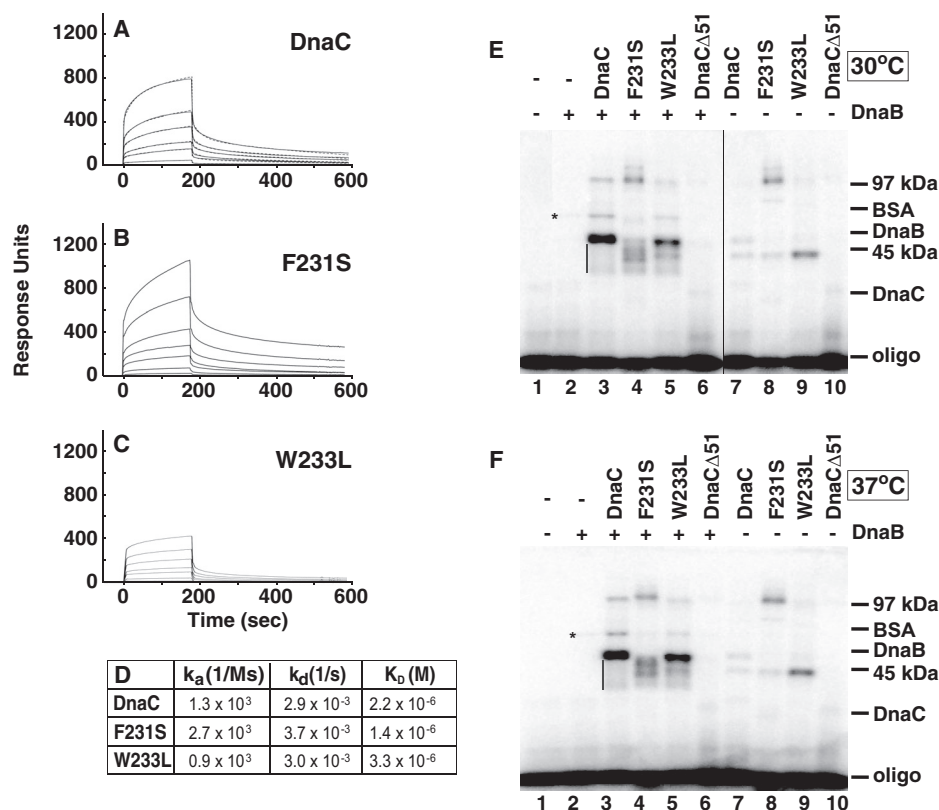
FIGURE 4. Compared with wild type DnaC, F231S and W233L interact aberrantly with ssDNA. A–C, the binding of wild type DnaC (A) or each mutant (B and C) at 0.6, 1.25, 2.5, 5, 7.5, and 10 \mu M to an oligonucleotide (CATCCAATAAATCATACACAAGGC in which the 5'-end was biotinylated, 400 response units) immobilized onto a streptavidin-coated sensor chip was measured using a Biacore 2000 biosensor (GE Healthcare) in buffer containing 50 mM HEPES-KOH, pH 8.0, 30 mM KCl, 5 mM MgCl 2 , 5% (v/v) glycerol, 0.002% (v/v) Tween 20, 4 mM DTT, and 2 mM ATP. Representative sensorgrams from two essentially identical analyses are shown in which the background signal from a flow cell that lacks streptavidin was subtracted. D, using BIAevaluation 3.1 software, kinetic constants and the equilibrium dissociation constant ( K_D ) of wild type DnaC were determined by fitting sensorgrams (A, dashed lines) to a global kinetic model. The sensorgrams obtained with F231S and W233L could not be fitted, so K_D values were estimated by separately fitting association and dissociation curves. E and F, UV cross-linking of a 5'-labeled oligonucleotide (60 fmol) with 0.4 \mu M DnaB (monomer) where indicated, and 2 \mu M of either DnaC, F231S, or W233L was performed essentially as described (29), but with minor modifications (see "Experimental Procedures"). DnaB, wild type DnaC, and the mutants of this experiment were isolated as described under "Experimental Procedures" in which the final step of purification was by gel permeation chromatography on Superose 12 or Superdex 75 10/30 columns, respectively (GE Healthcare). DnaB eluted at the position expected for hexameric DnaB; DnaC and the mutants eluted at the position of monomeric DnaC. Following cross-linking at 30 or 37 °C, molecular weight markers (phosphorylase B (97 kDa), BSA (68 kDa), DnaB (52 kDa), ovalbumin (45 kDa), and DnaC (28 kDa)) separated by SDS-polyacrylamide gel electrophoresis were detected by Coomassie Brilliant Blue staining before autoradiography. The asterisk indicates the position of DnaB cross-linked to the oligonucleotide. In E, lanes 2–6 were rearranged by image editing for consistency with F. Results similar to those presented here were obtained in five essentially identical experiments.
