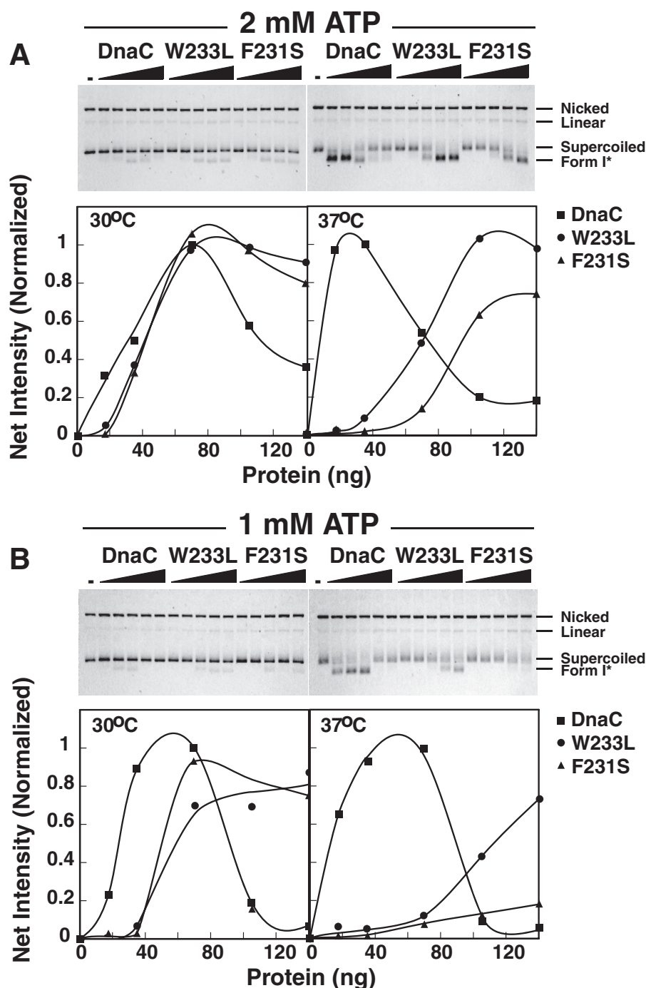
FIGURE 6. F231S and W233L are thermolabile in the formation of a highly negatively supercoiled DNA named Form I*. Reactions (25 \mu l) contained 2 mM (A) or 1 mM (B) of ATP, DnaC, F231S, or W233L, a supercoiled plasmid carrying oriC (M13oriC2LB5, 200 ng), HU, single-stranded DNA-binding protein, DnaA, DnaB, and DNA gyrase as described (44). After incubation for 25 min at 30 or 37 °C, SDS and EDTA were added to final concentrations of 1% and 10 mM, respectively and then incubated for 4 min at 65 °C. After agarose gel electrophoresis, the electrophoretically separated DNAs were visualized by ethidium bromide staining. The reverse images are shown in which the leftmost lanes of each gel lack DnaC. In addition, the amounts of Form I* were quantified and normalized relative to the optimal level observed with wild type DnaC.
