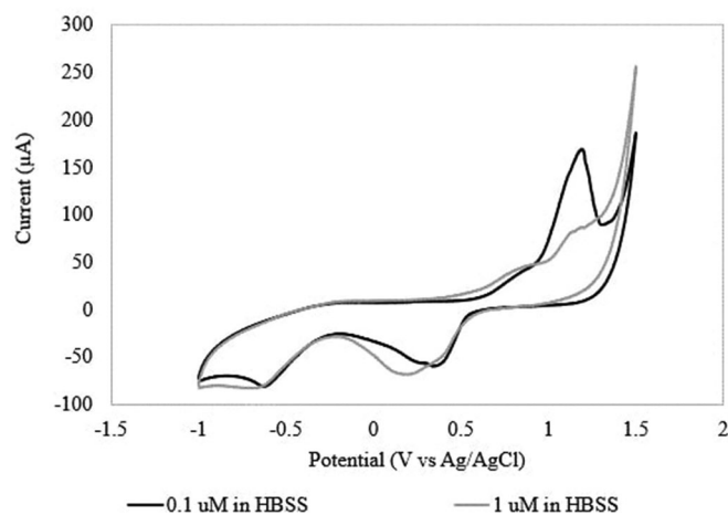
Figure 2. CV curves of 0.1 \mu\text{M} \text{H}_2\text{O}_2 in HBSS and 1 \mu\text{M} \text{H}_2\text{O}_2 in HBSS.
