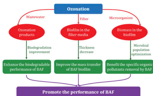
Figure 6. The positive influence of ozonation on the performance of BAF in ozonation-BAF process. Adapted from Ref. [93].
