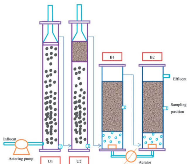
Figure 5. Technological scheme of combined UASB/BAF. Adapted from Ref. [61].
