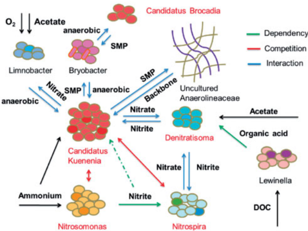
Figure 4. Proposed interactions between key functional nitrogen removal guilds in SNAD-IFAS process. Adapted from Ref. [59].
