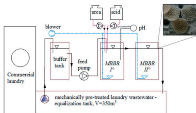
Figure 1. Technological scheme of MBBR. Adapted from Ref. [25].
