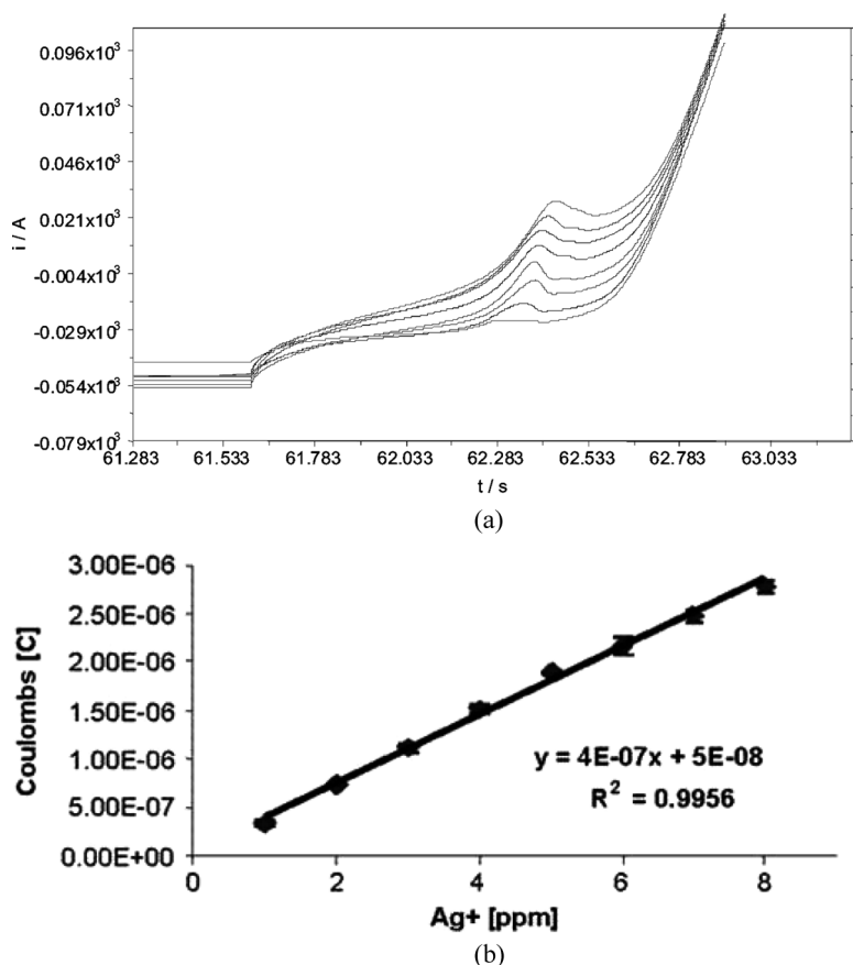
Figure 3. A calibration curve and spectra for the electrochemical measurement of silver ions in the presence of ferricyanide and thiocyanate vs a carbon ammonium thiocyanate ferri/ferro cyanide reference element (a) the recorded scans and (b) the graph of the integration under the peaks against concentration of silver ions in ppm.
