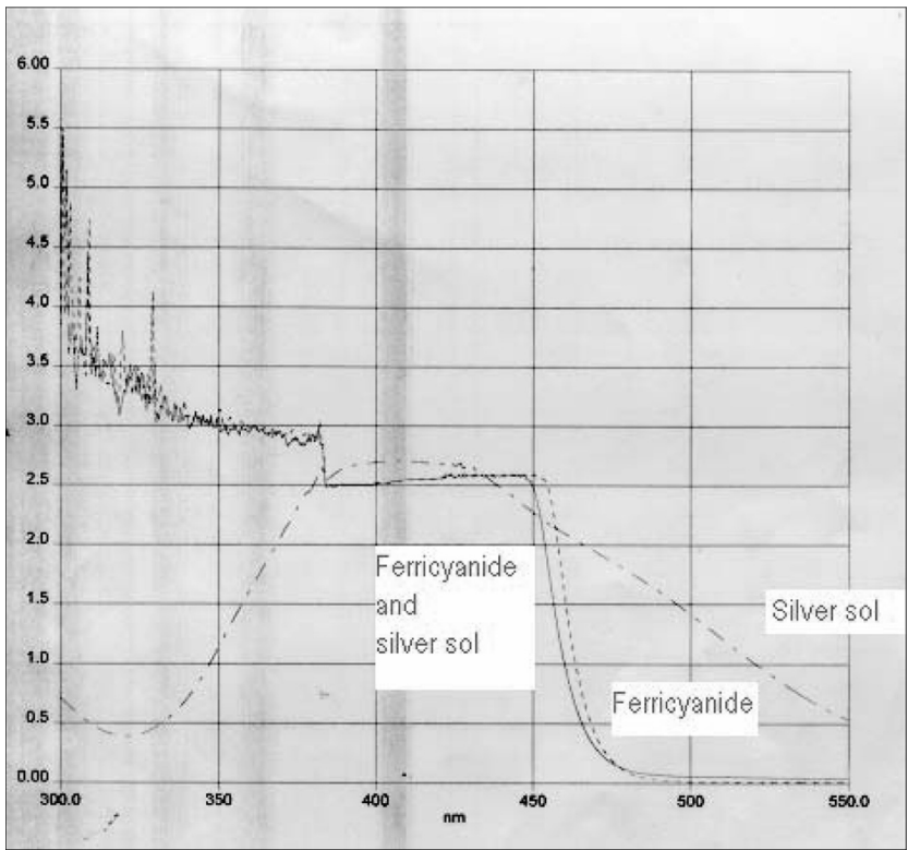
Figure 5. UV spectrometric data showing the that silver sol is dissolved using ferricyanide in water.
