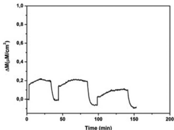
Figure 9. Reproducibility of MIP QCM biosensor. Experimental conditions; pH 7.4, flow rate: 1.0 mL/min, concentration of L-histidine: 96.6 μM.
