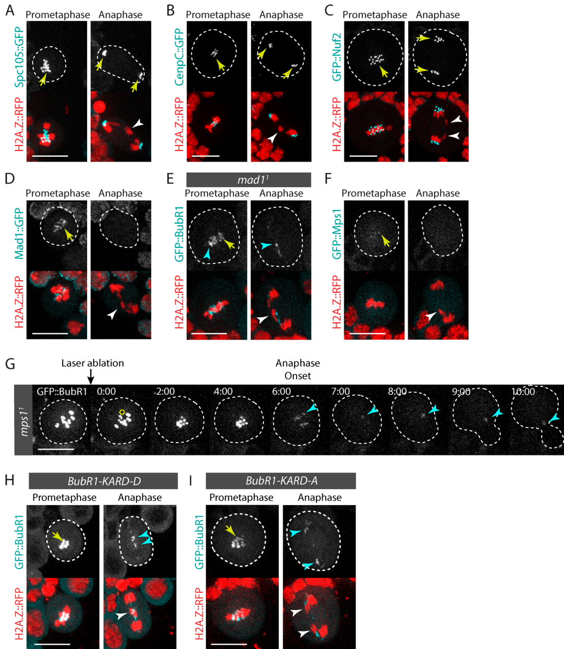
Figure 3. DNA breaks do not induce neokinetochore formation. (A–D and F) Time-lapse images of neuroblasts expressing H2A::Z::RFP and Spc105::GFP (A), CenpC::GFP (B), GFP::Nuf2 (C), Mad1::GFP (D), and GFP::Mps1 (F) after I-Cre expression. The white arrowheads point to the I-Cre-induced acentric chromatids. Yellow arrows indicate the localization of the GFP-labeled proteins at the kinetochore. (E) Mad1 is not required for BubR1 localization on broken chromatids. Time-lapse images of a mad1 1 mutant neuroblast expressing I-Cre and labeled with H2A::Z::RFP and GFP::BubR1. The white arrowhead indicates I-Cre-induced acentric chromatids. The yellow arrow and cyan arrowheads indicate the localization of GFP::BubR1 at the kinetochore and tether. (G) Mps1 is not required for BubR1 localization on broken chromatids. Time-lapse images of mps1 1 mutant neuroblast labeled with GFP::BubR1 before and after laser ablation. The yellow circle corresponds to the zone of laser ablation. The cyan arrowheads indicate the appearance of GFP::BubR1 at the site of chromosome damage. Time (given in minutes/seconds) 0:00 corresponds to the first acquisition immediately after laser ablation. (H and I) BubR1 localization on DNA breaks does not require Polo-dependent phosphorylation of the BubR1 KARD motif. Time-lapse images of neuroblasts expressing I-Cre labeled with H2A::Z::RFP. The neuroblasts express either the GFP::BubR1-KARD-D mutant, where the putative Polo-dependent phosphorylation sites in the KARD motif are replaced by aspartate (H), or GFP::BubR1-KARD-A, where the same residues are mutated to alanine (I). The white arrowheads indicate the I-Cre-induced acentric chromatids. Yellow arrows and cyan arrowheads point to the localization of GFP::BubR1-KARD-D and GFP::BubR1-KARD-A on the kinetochore and tether. Cells are delineated with white dotted lines. Bars, 10 \mu m.
