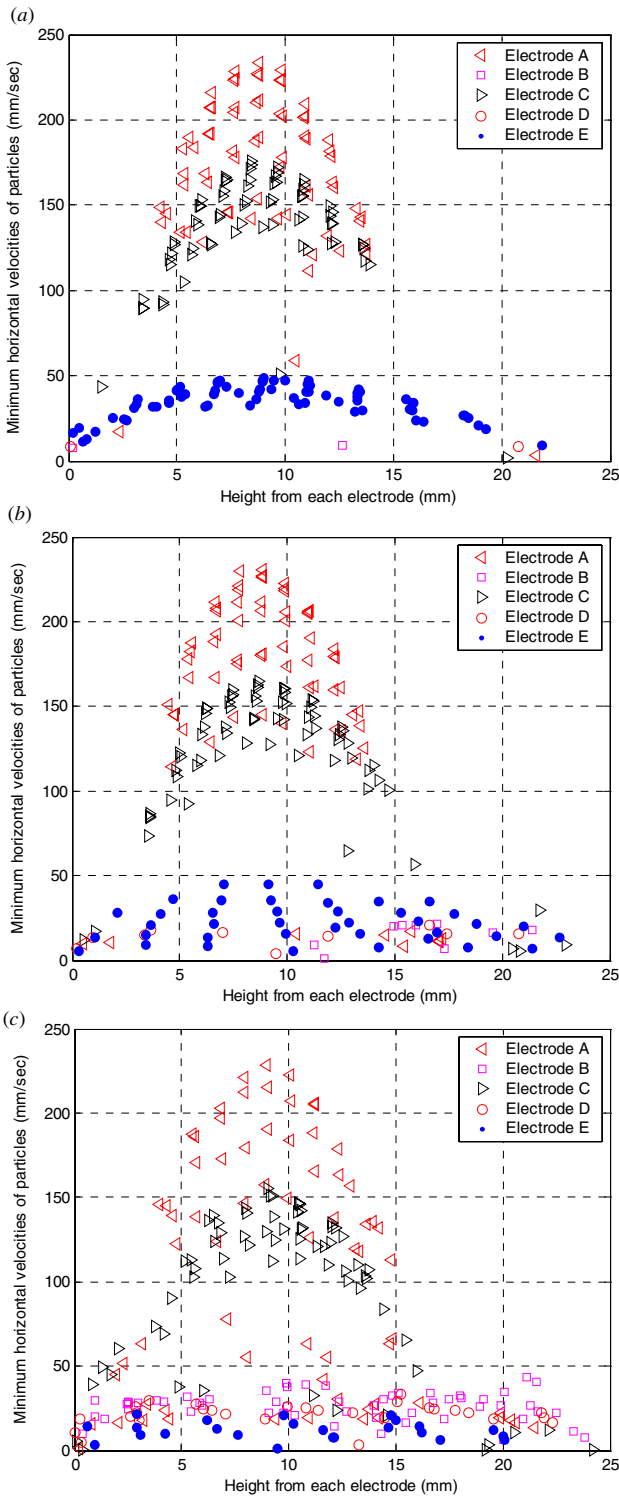
Figure 4. Minimum horizontal velocities of the particles passing through the expanded volumes versus the distance of the particles from each electrode at a flow rate of 1.1 l min -1 in the SO (a), BO (b) and FO (Jang et al 2007) (c) configurations.
