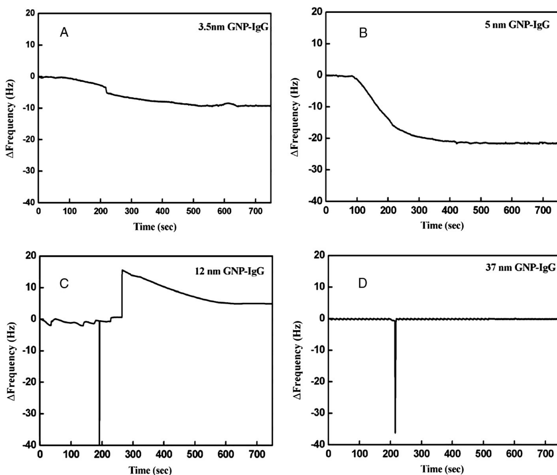
Figure 3. Detection of GNPs using an anti-5 nm GNP antiserum-coated QCM. The frequency shift was monitored for injection of 5 \mu l of (A) 3.5 nm GNPs, (B) 5 nm GNPs, (C) 12 nm GNPs, and (D) 37 nm GNPs. The concentration of GNPs was 0.1 mM. The switching action of the injector occasionally caused spikes during the detection.
