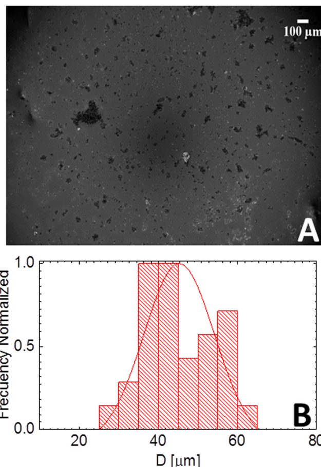
Figure 3. (A) SEM image showing the resulting overall coverage of the Pt electrode after the deposition of the ZnO NW/graphite film fragments. (B) Histogram of approximate fragment sizes.
