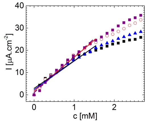
Figure 10. Degree of reproducibility of biosensor electrodes as examined by comparing various independently determined calibration curves.
