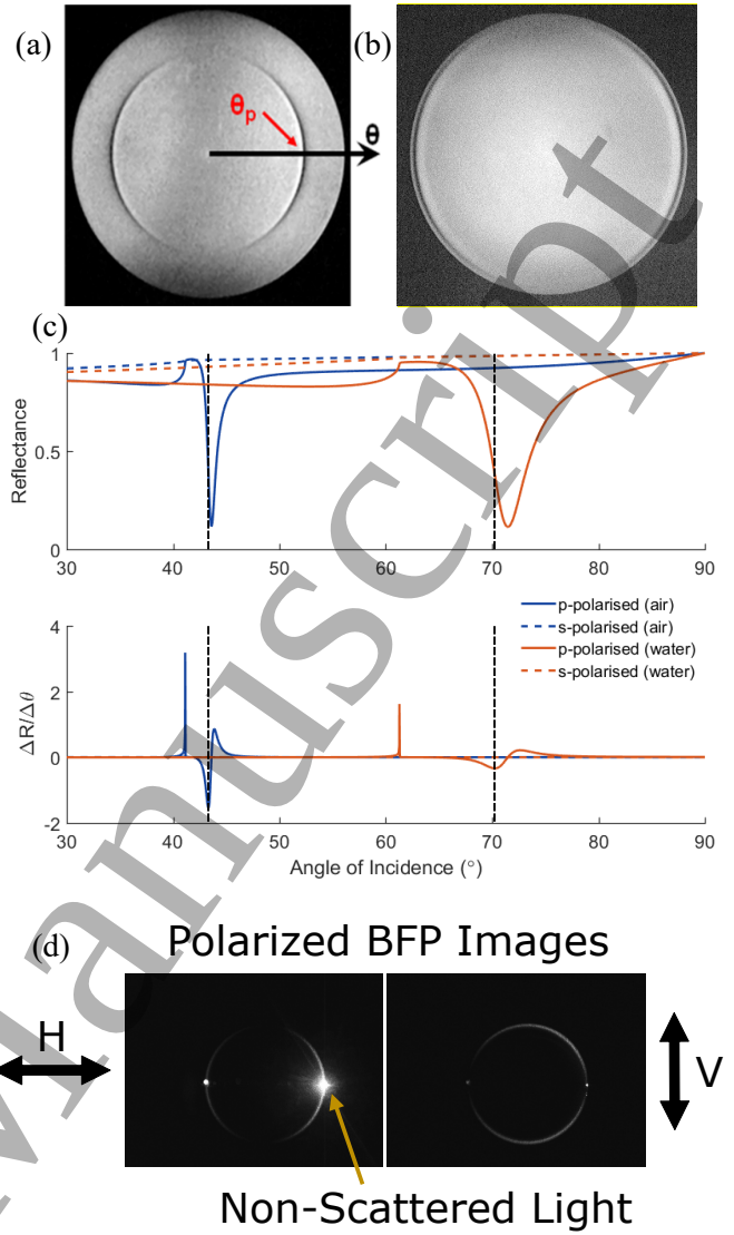
Figure 3. Images of a uniformly illuminated back focal plane, with the gold sample in air (a) and water (b). The dark arcs indicate the angles at which plasmon resonance occur. Note that only p -polarized light can excite plasmons, which is why arcs appear and not a ring. (c) Theoretical angular SPR response for p - and s -polarized light with air and water as the dielectric. S -polarized light is not capable of exciting surface plasmons. Using p -polarized light and increasing the refractive index of the dielectric increases the angle where resonance occurs. The angle where the gradient ( \Delta R/\Delta\theta ) is greatest is marked on each curve. (d) Images of the back focal plane imaged through a polariser with cells growing on a gold SPR surface. Note that light scattered off refractive index discontinuities in the sample returns from the same elevation angle but all azimuthal angles. This illustrates that momentum is conserved during plasmon scattering.
