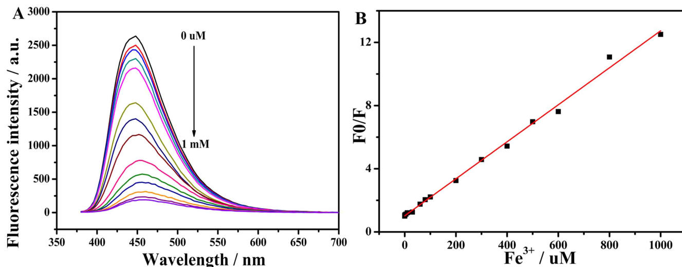
Figure 7. (A) Fluorescence spectra of the N-CQDs after treatment with different concentrations of Fe 3+ (0–1000 \mu M) in the real sample. (B) Linear relationship between the F0/F and Fe 3+ concentration.
