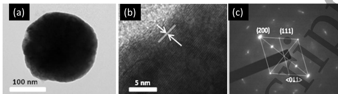
Figure 2: TEM images (a), with high-magnification (b), and SAED patterns (c) of cubic \text{Cu}_2\text{O} .
